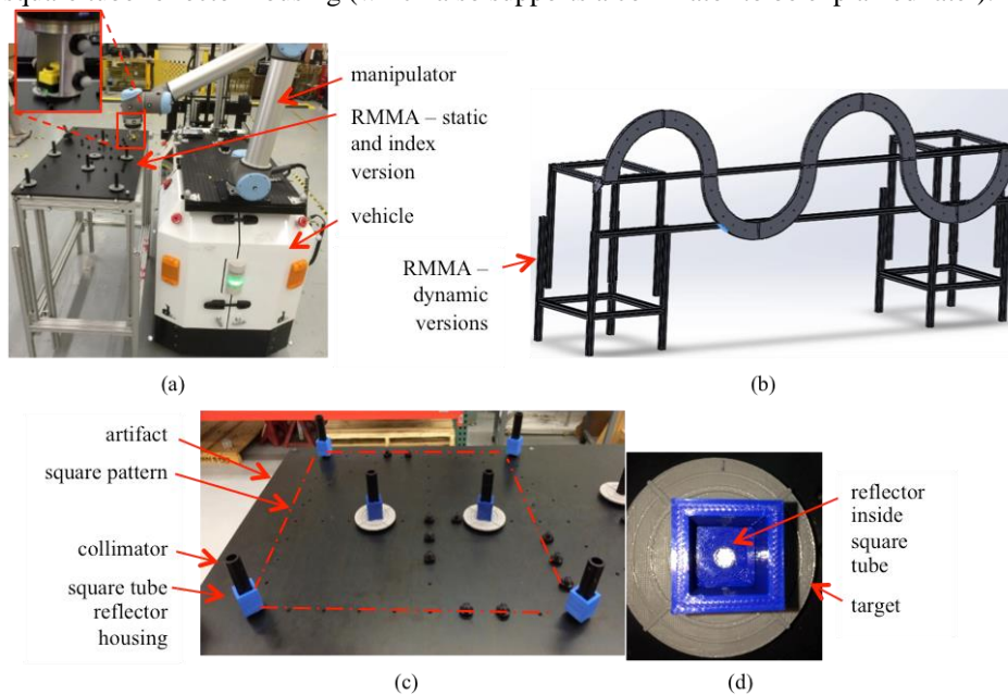
Figure 1: Reconfigurable mobile manipulator artifacts (RMMAs) showing (a) static and index version (RMMA-1) and (b) dynamic version (RMMA-2). (c) Static and index version square pattern of reflectors and (d) close-up, top view of an illuminated reflector inside the square tube. The inset in (a) shows the retroreflective laser sensor used to detect reflectors.
