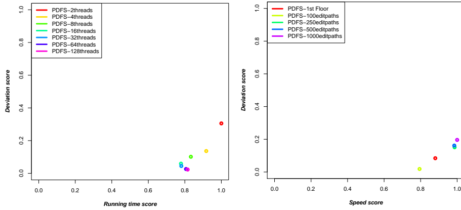
Fig. 3. Time-deviation score: Left (#Threads), right (# Edit Paths).
