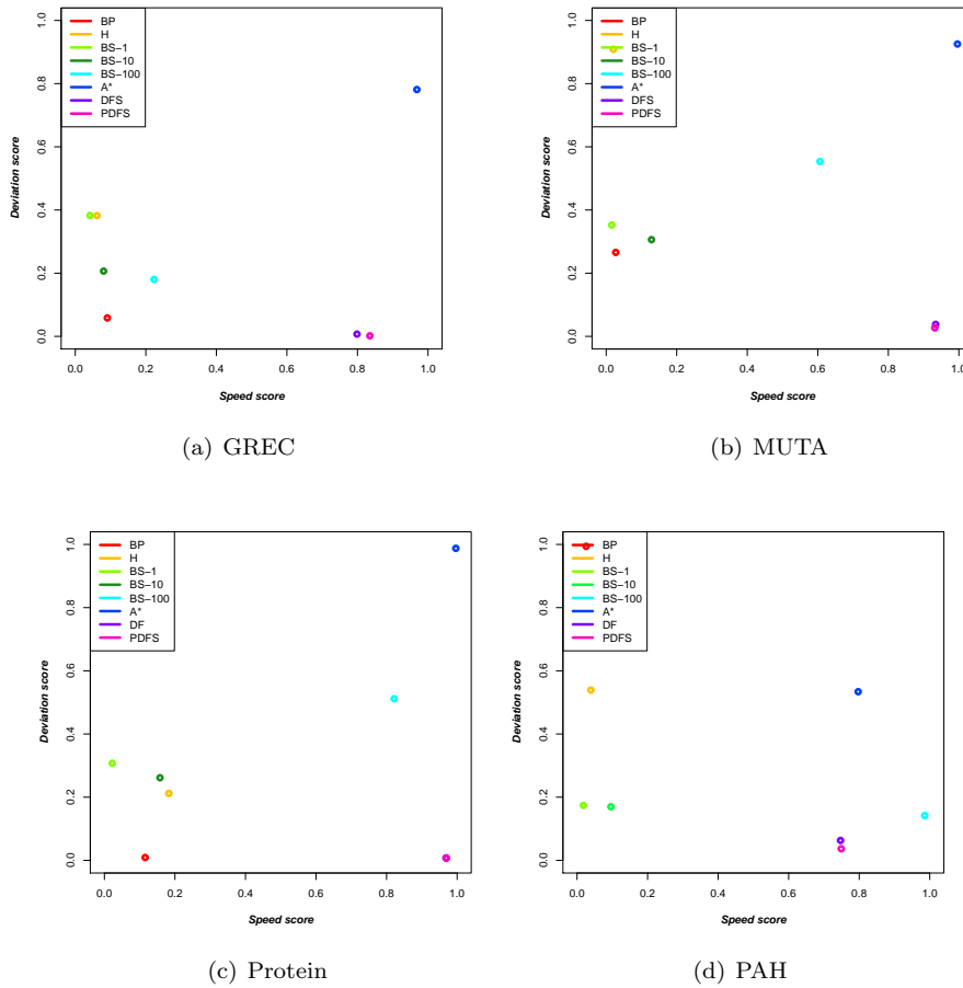
Fig. 8. Time-deviation score under small time constraint.
