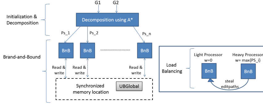
Fig. 2. The main Steps of PDFS
