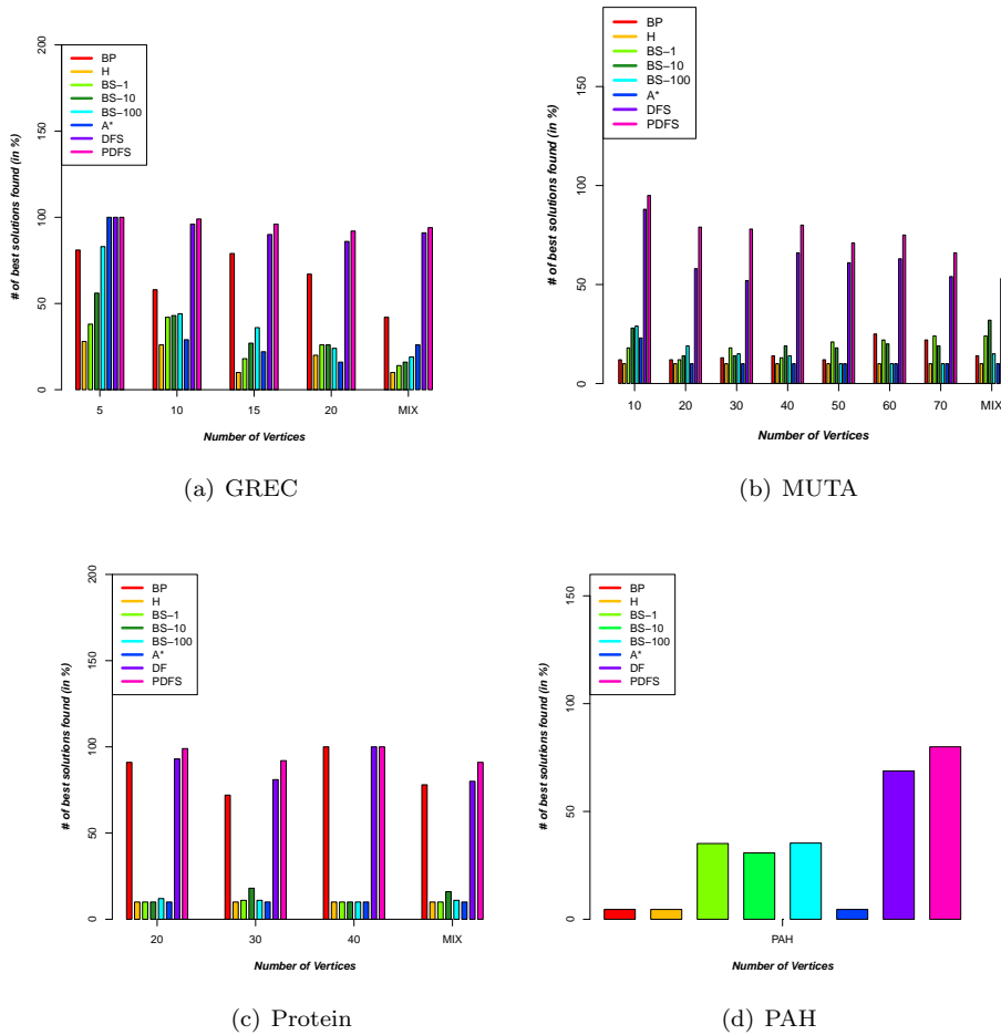
Fig. 7. Number of best found solution under small time Constraint
