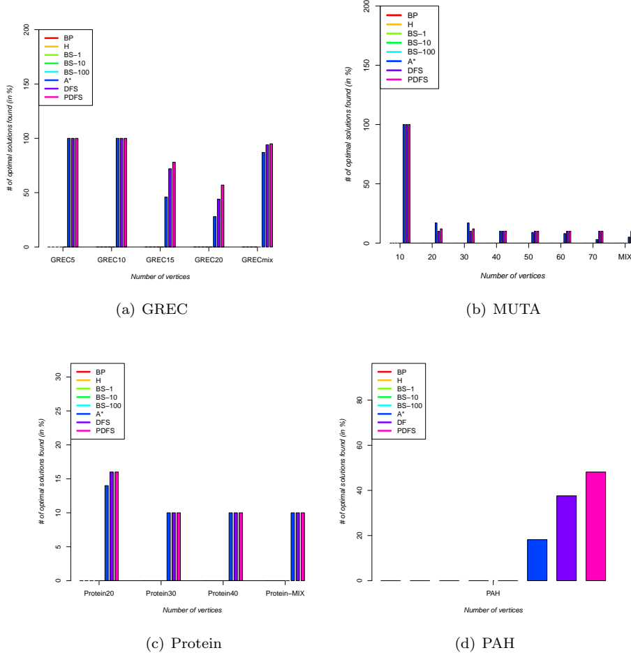
Fig. 5. Number of optimal solutions under big time constraint
