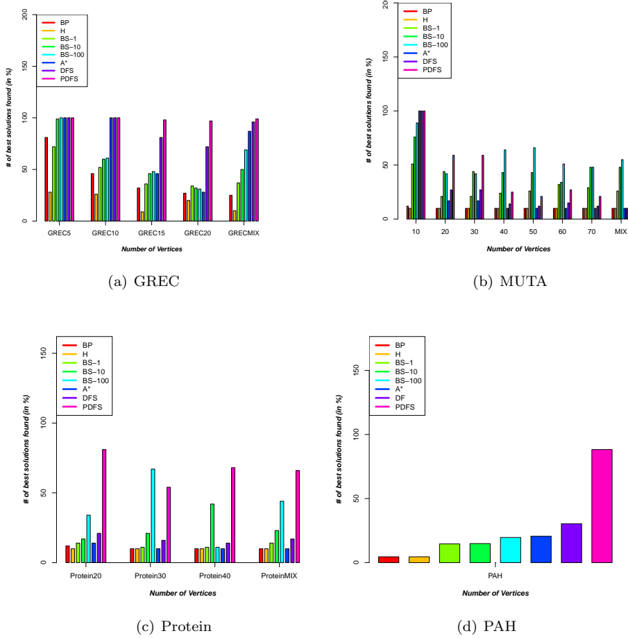
Fig. 4. Number of best found solution under big time constraint
