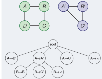
Fig. 1. An incomplete search tree example for solving the GED problem. The first floor represents possible matchings of vertex A with each vertex of the second graph (in blue). A tree node is a partial solution which is to say a partial edit path.
