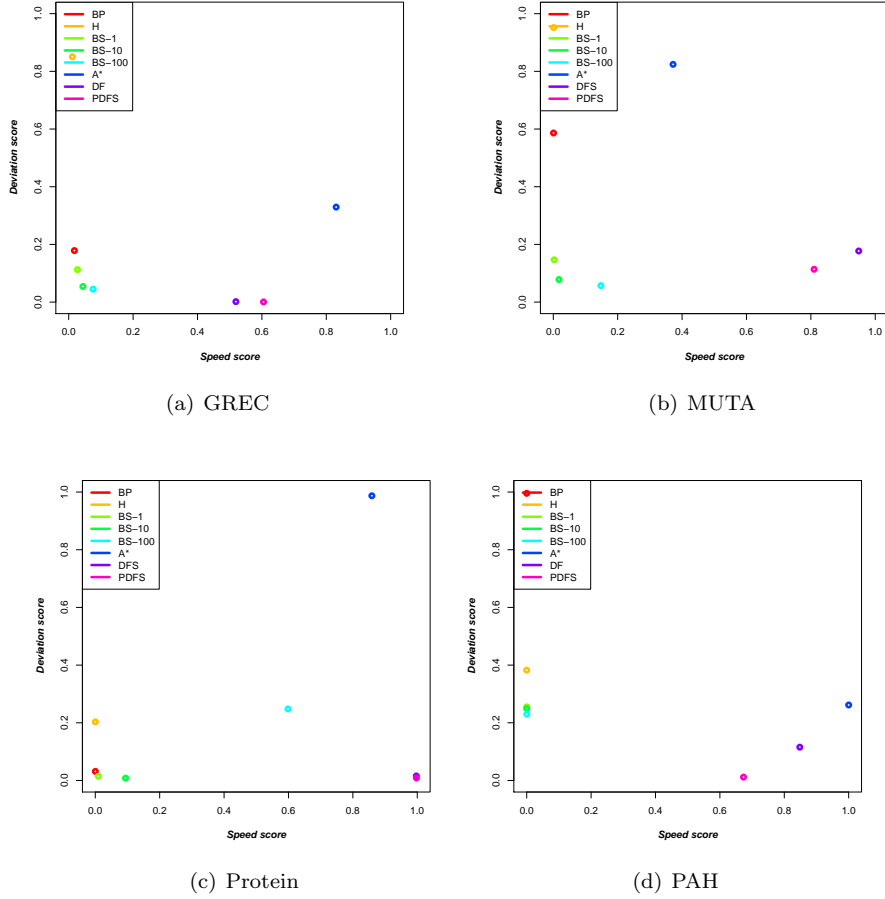
Fig. 6. Time-deviation score under large time constraint
