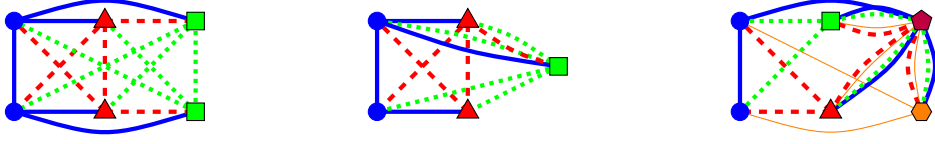
Figure 7: Three completely independent spanning trees of K_6 (on the left), three (0, 2) -disjoint spanning trees of K_5 (on the middle) and four (1, 3) -disjoint spanning trees of K_6 (on the right) (thin line: edge of T_4 ; hexagon: I(T_4) ; pentagon: I(T_1) \cap I(T_2) \cap I(T_3) \cap I(T_4) ).
