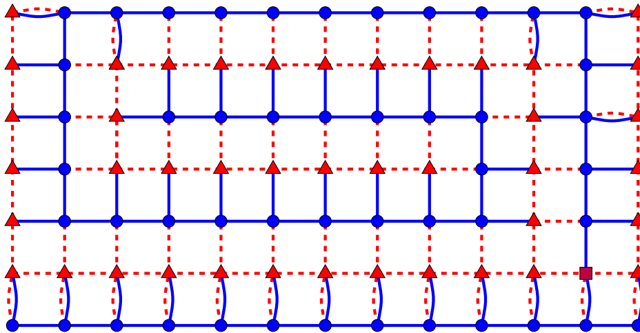
Figure 9: Two (1, 18) -disjoint spanning trees of G(7, 13) .
