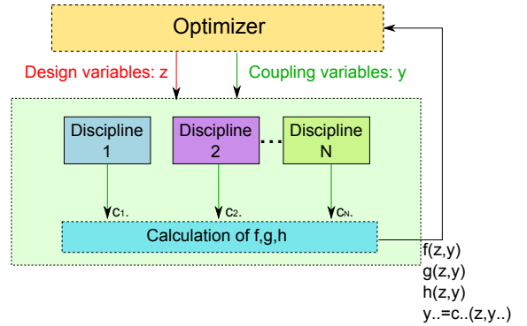
Figure 8: Multidisciplinary Design Optimization, decoupled approach
