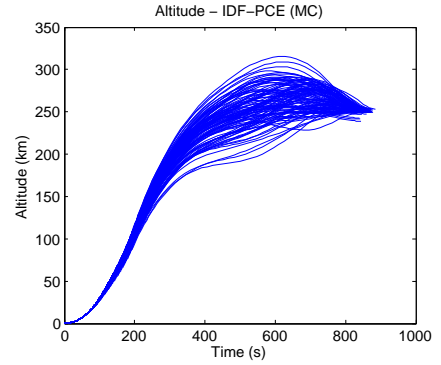
Figure 26: Optimal trajectory altitude under uncertainty - IDF-PCE
