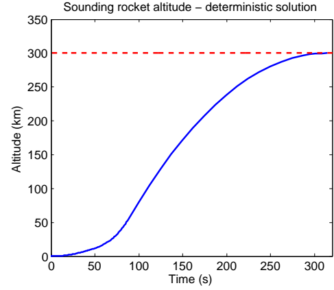
Figure 32: Optimal sounding rocket altitude without uncertainty
