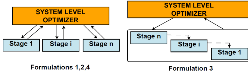
Figure 10: SWORD formulations (formulations 1,2,4 are parallel and formulation 3 is hierarchical)
