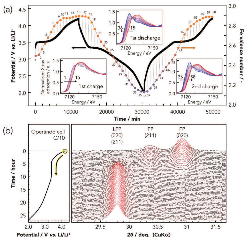
Fig. 5 In situ XAFS and XRD measurements on a half-cell consisting of Li/1 M \text{LiPF}_6 EC + DEC (LFP/graphitic carbon) composites. (a) Solid bold line shows the galvanostatic charge profile of LFP/graphitic carbon during the in situ XANES measurements at 0.1C. Dashed lines correspond to the changes in the evaluated “formal valence number” of Fe during the lithiation–delithiation process. The formal valence number of Fe for the composites was calculated by fitting using commercial \text{LiFePO}_4 powder and \text{FePO}_4 powder oxidized using the chemical method. The XANES spectra at the iron K-edge of \text{Li}_x\text{FePO}_4 are shown in three insets. (b) Detailed XRD patterns during the second discharge reactions for the 0.1C rate. The voltage profiles during the measurements are shown on the left.
