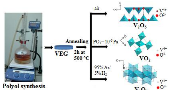
FIGURE 1. Scheme of the polyol process used for the synthesis of vanadium pentoxide V 2 O 5 , vanadium dioxide VO 2 and vanadium sesquioxide V 2 O 3 powders.
