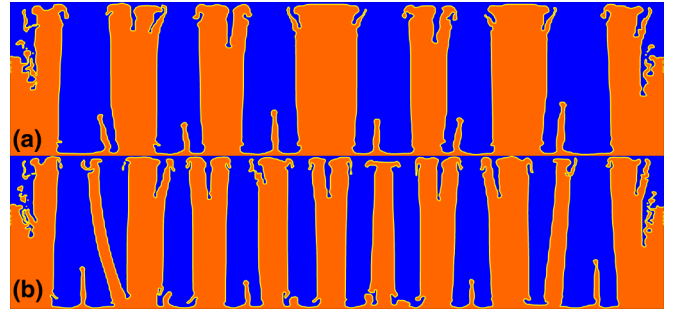
FIG. 7. Evolution of quasistationary band patterns calculated for zero surface tension with the decrease of dynamic viscosity (same for both fluids) (a) \eta = 0.075 Pa.s, (b) \eta = 0.05 Pa.s. Vibration characteristics are f = 30 Hz, a = 1.8 mm.
