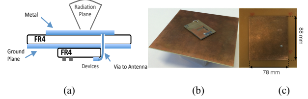
Fig. 9. Dual-band rectenna : Schematic (a) Rectenna back side (b) and front side (c)
