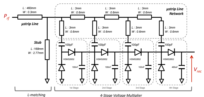
Fig. 1. Architecture of the RF to DC converter
