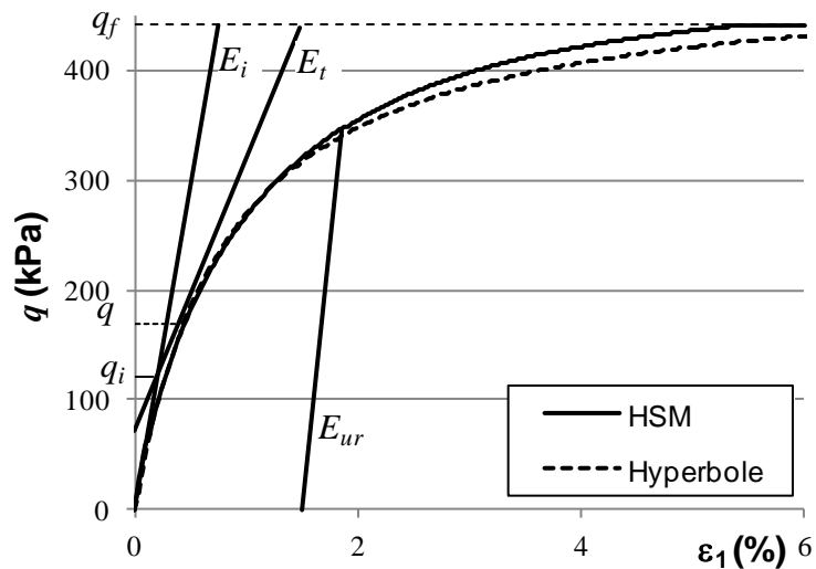
Figure 3. Essai triaxial HSM et hyperbole
