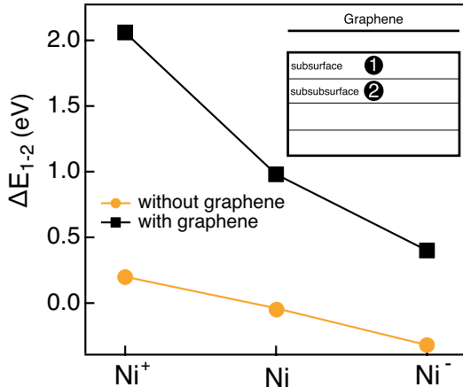
FIG. 5. Differences in carbon dissolution energies ( \Delta E_{1-2} ), for a carbon atom located in subsurface (1) or sub-subsurface (2) interstitial site, without (yellow) and with (black) graphene covering a (111) slab of "nickel" with different C solubilities. Inset: Sketch of the epitaxial graphene covered (111) slab, with the interstitial sites indicated.
