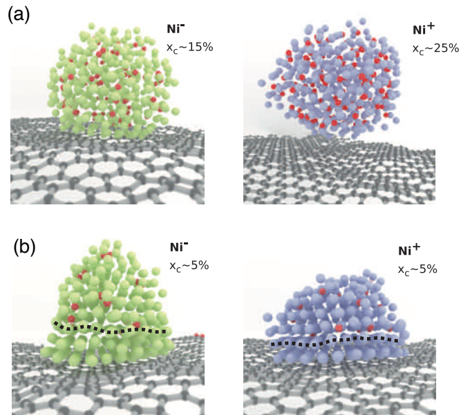
FIG. 4. Probing the wetting of carbon-containing metal nanoparticles deposited on graphene (a) Equilibrium structures corresponding to C-saturated NPs. \text{Ni}^- NP (left) shows a contact angle slightly larger than 90^\circ , while \text{Ni}^+ NP (right) is fully dewetting the substrate. (b) At intermediate concentration, we observe a carbon depletion close to the graphene layer. This absence of carbon dissolved close to the contact is more pronounced for \text{Ni}^- (left), with two pure metal layers than with \text{Ni}^+ (right). Dashed lines delimit the C-depleted metal zone. \text{Ni}^- atoms are green, \text{Ni}^+ atoms are blue, C atoms inside the NP are red.
