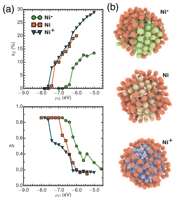
FIG. 3. (a) Top : C adsorption isotherms as a function of \mu_c . Bottom : average values of the order parameter as a function of \mu_c for a NP initially Wulff shaped with 405 atoms. (b) Snapshot of characteristic configurations for metal-C NPs ( \text{Ni}^- green, Ni beige and \text{Ni}^+ , blue atoms) surrounded by a disordered shell (orange atoms). Black balls correspond to C atoms.
