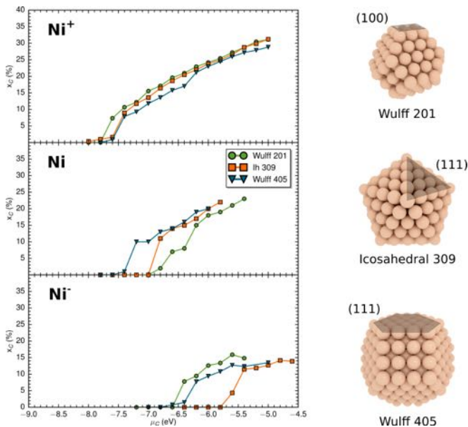
FIG. 2. (Left) Carbon adsorption isotherms calculated at T = 1000K on the basis of GCMC simulations for NPs (with 201, 309 and 405 atoms) with high (top) and low (bottom) carbon solubility. (Right) Schematic representation of Wulff and Ih structures where the different facets are presented. The NP with 309 atoms is Ih when pure, the others are FCC, with their Wulff equilibrium shape.
