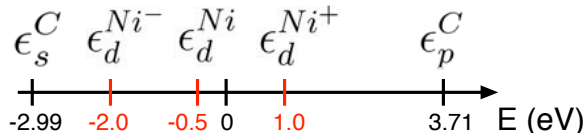
FIG. 1. Schematic representation of the atomic levels used in our tight-binding model.
