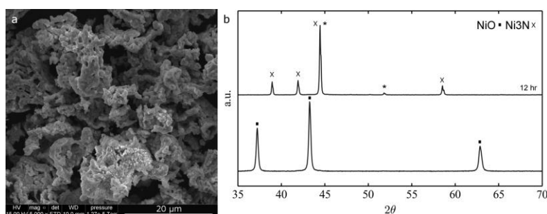
Figure 9. SEM micrograph of a sponge-like \text{Ni}_3\text{N} structure (obtained from \text{NiO} nanofibers derived from PVP and nickel acetate in DMF/ethanol) (a) and the corresponding XRD diffractogram (b) before and after the two-step complete conversion in \text{NH}_3 . JCPDS reference: \text{Ni}_3\text{N} 00-010-280, Ni 96-151-2527.
