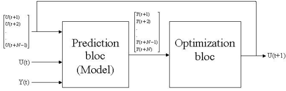
Fig. 4. Traffic regulator based on Model Predictive Control
