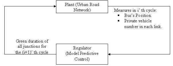
Fig. 3. Control architecture of the traffic process
