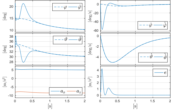
(b) Observer Results: Only the first two seconds are shown since after this time the estimation follows the state with high fidelity for all the rest of the simulation.
