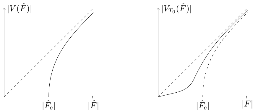
(A) No thermal noise: stick-slip law. (B) With thermal noise: Arrhenius law.
