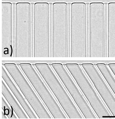
FIG. 1: Lamellar eutectic patterns observed in situ during thin-sample directional solidification ( V = 0.5 \mu m s^{-1} ) of a eutectic transparent ( CBr_4-C_2Cl_6 ) model alloy. a) Symmetric steady-state in a “floating” eutectic grain. b) Tilted lamellae in a “locked” eutectic grain. The growth direction is vertical (liquid on top). Bar: 20 \mu m .
