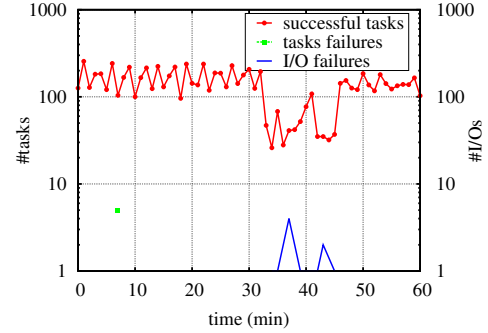
Figure 5. Successful vs. failed MapReduce tasks
