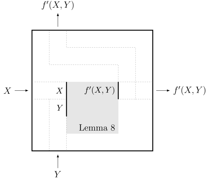
Figure 4: A block simulating the local transition function of a 1D CA.
