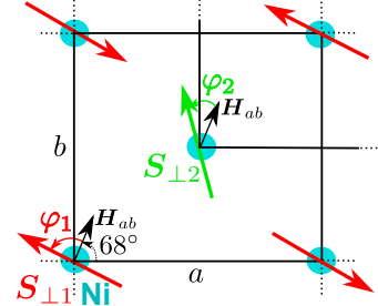
FIG. S6. Sketch of a general magnetic structure (orientations of \mathbf{S}_{\perp 1} and \mathbf{S}_{\perp 2} vectors) that was anticipated in the fits. Crystallographic ab plane corresponds to the plane of the figure, and \mathbf{H}_{ab} is the projection of the field into this plane (its orientation, at 68^\circ from the a axis, was determined from the fit of the nitrogen quadrupolar splittings - see the text). Red and green colors denotes the two different tetragonal subsystems present within the BCT lattice. For the final solution (A in Tab. III), \mathbf{S}_{\perp 1} and \mathbf{S}_{\perp 2} are found to be mutually parallel and nearly perpendicular to \mathbf{H}_{ab} ( \varphi_1 = \varphi_2 = 96(4)^\circ ).
