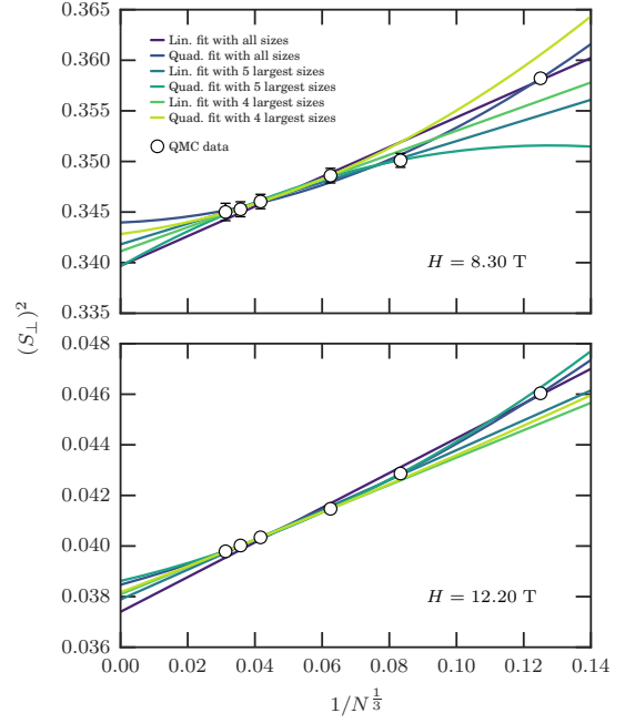
FIG. S1. Two examples, at different magnetic fields, for the extrapolation of the order parameter to the thermodynamic limit. Various linear and quadratic fits (solid lines) are performed taking into account a varying number of QMC data points (circles). SSE simulations are performed for the DTN model at T = 0.12 K.
