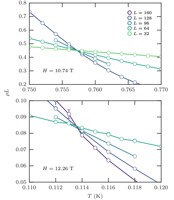
FIG. S2. Two examples, at different magnetic fields, of the crossing of the spin stiffness \rho times the system size L to determine the critical temperature.
