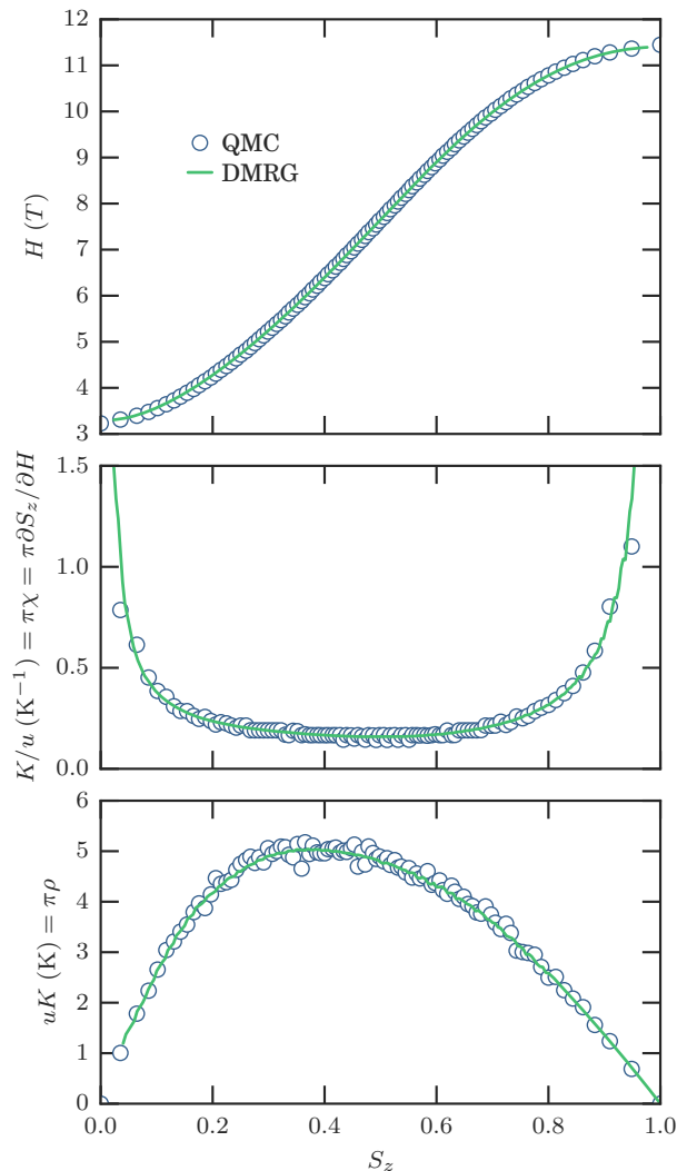
FIG. S4. Comparison between QMC (circles) and DMRG (lines) results to determine the values of u and K . The susceptibility \chi is the first derivative of the magnetization curve S_z(H) and \rho is the spin stiffness. QMC error bars are smaller than the symbol size and thus not visible. Note that the critical fields observed in the first panel are purely one-dimensional.
