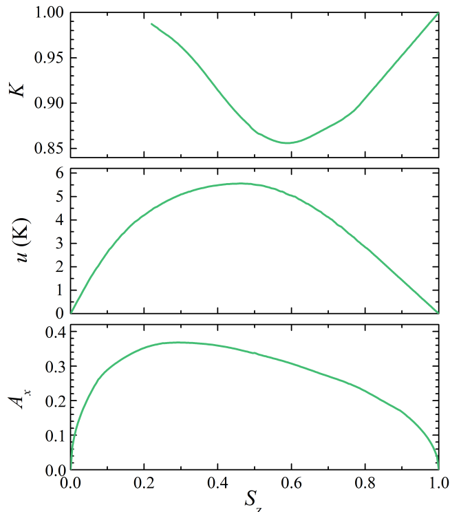
FIG. S3. TLL parameters as a function of sample magnetization S_z , calculated by DMRG for the DTN ( J_c = 2.2 K, D = 8.9 K). Values for K at S_z \rightarrow 0 are not represented as the behavior of K in that region could not be precisely defined.
