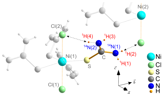
FIG. S5. Location of the ^1\text{H} (red) and ^{14}\text{N} (blue) NMR sites within the unit cell in DTN. The Ni(1) and Ni(2) nickels seen on this figure belong to the 2 different tetragonal subsystems. Dashed double arrows indicate hydrogen bonds.
