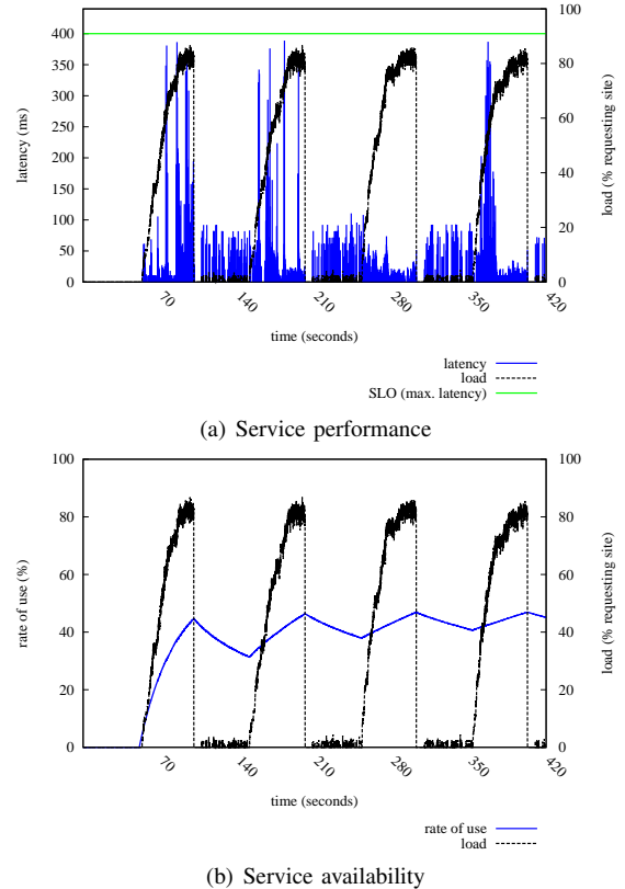
Figure 11. Self-adaptive locking service
