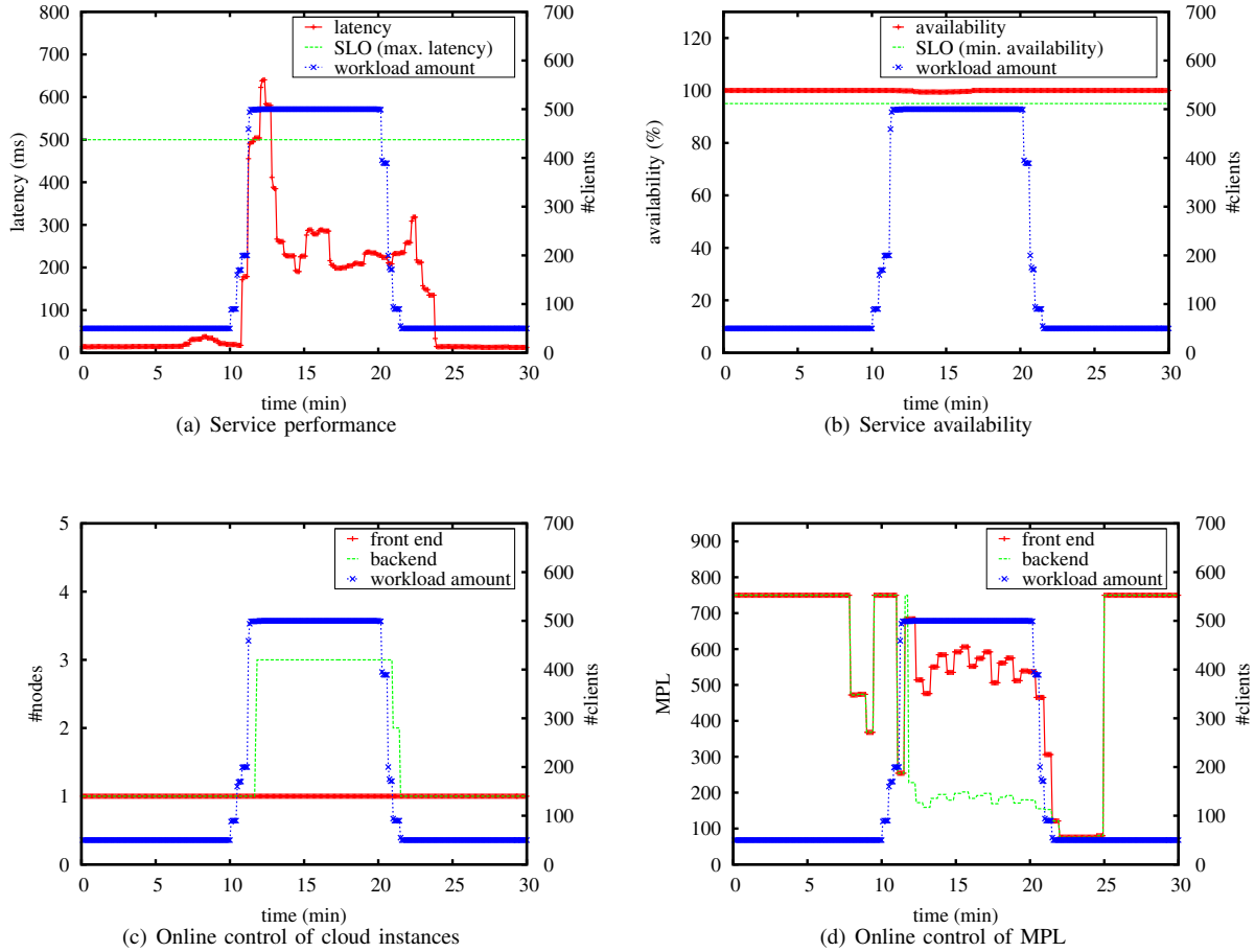
Figure 9. Self-elastic multi-tier bookstore service
