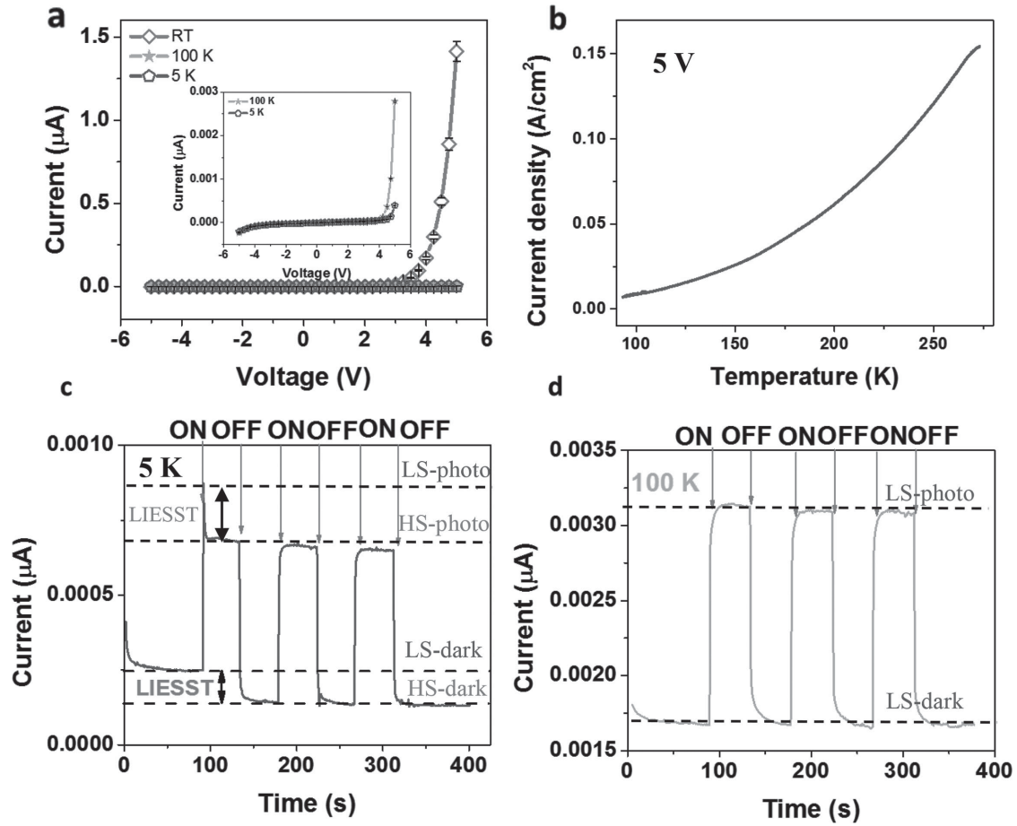
Figure 4. Electrical characteristics of a 30 nm junction. a) I - V curves registered at room temperature, 100 and 5 K at a rate of 100 mV \text{s}^{-1} . The inset is a zoom on the 100 and 5 K data. b) Temperature dependence of the conductivity of the junction registered at a rate of 5 K \text{min}^{-1} . c,d) Visible light irradiation effect on the current flowing in the junction through three successive ON/OFF cycles at 5 K (c) and 100 K (d). Current intensities in the HS and LS states are indicated by dashed lines both in dark and in photostationary conditions. The applied bias in (b–d) was 5 V.
