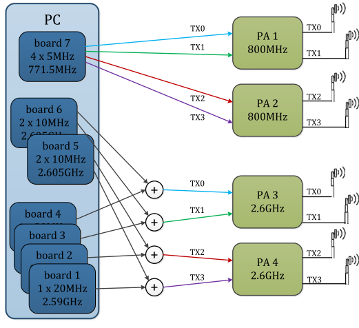
Fig. 4. Schematics of the transmitter.
