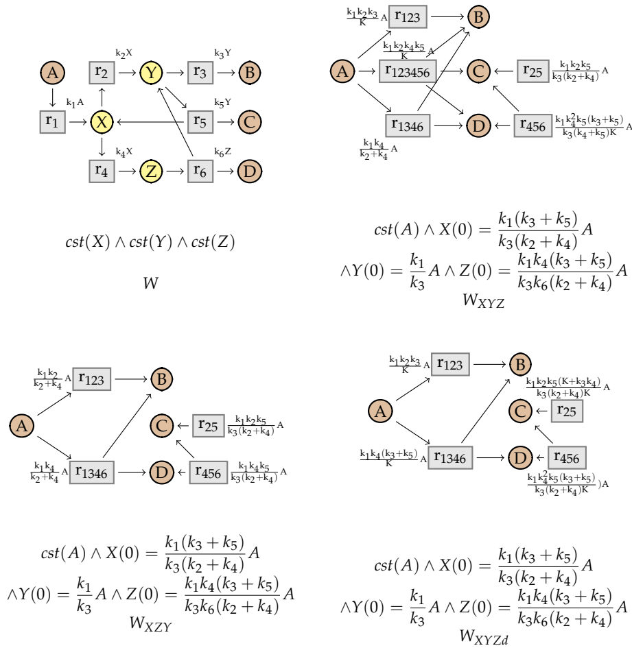
Figure 18. Network W and its simplifications. Top left: network W . Top right: network W_{XYZ} after eliminating X , Y and Z (in this order). Bottom left: network W_{XZY} after eliminating X , Z and Y . Bottom right: network W_{XYZd} after eliminating X , Y , Z , and the dependent reaction. The new parameter is K = k_2 k_3 + k_3 k_4 + k_4 k_5 .
