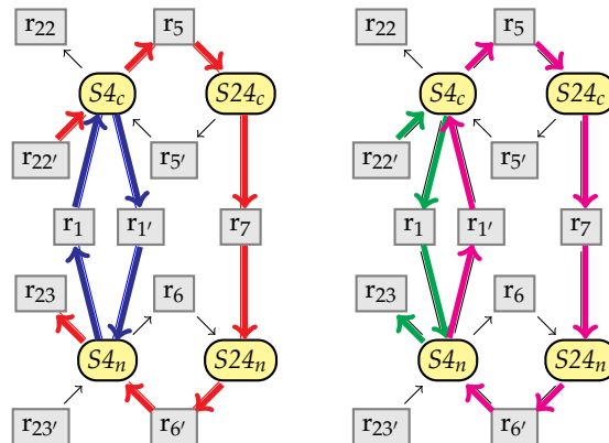
Figure 22. In red the elementary mode v_{red} , in blue v_{blue} , in green v_{green} , and in magenta v_{magenta} .
