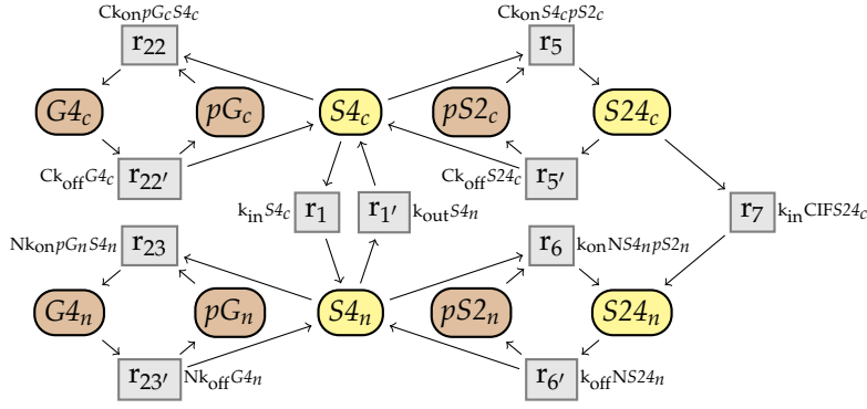
Figure 20. Sub-network W of the Smad -based signal transduction model from [23].
