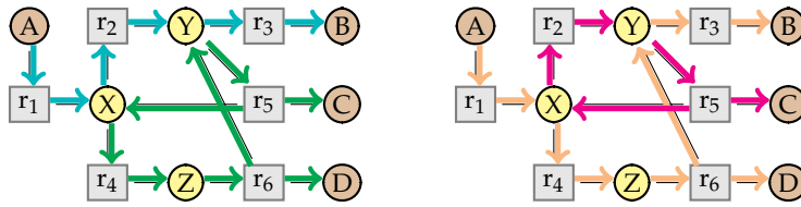
Figure 19. Two decompositions of the mode (1, 1, 1, 1, 1, 1) in the network W .
