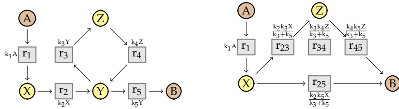
Figure 24. Networks W_0 (left) and W (right).
