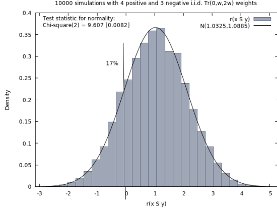
Figure 3. Distribution of outranking credibility \tilde{r}(x \succ y)
