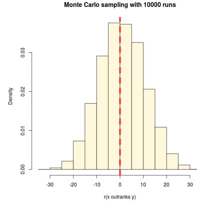
Figure 4. Distribution of outranking credibility \tilde{r}(a_1 \succ a_2)
