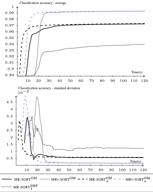
Figure 4. Average classification accuracy (top) and standard deviation (bottom) results over first set of benchmarks with 1,000 alternatives;
