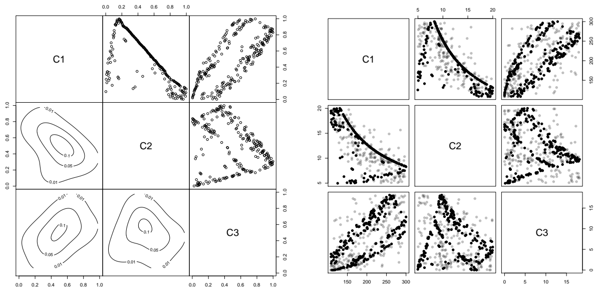
Figure 3: Peach ideotypes dataset. On the right, the pairs plot of the data points (black dots) and simulated points (gray dots). On the left, the original data points are represented as normalized ranks on the upper triangle and the estimated pair copulas as shown as contour plots on the lower triangle.
