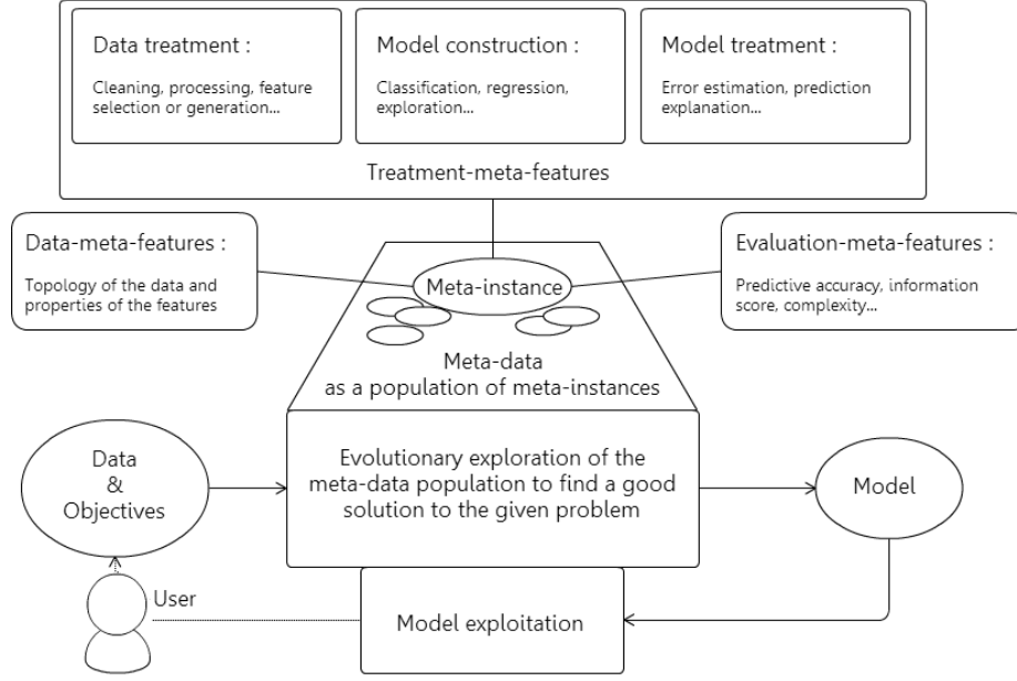
Figure 1: Modeling assistant
