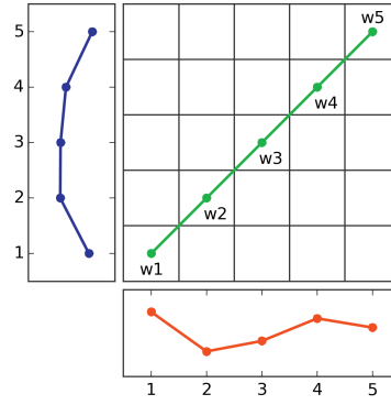
(b) Euclidean warping path
