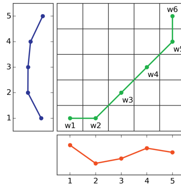
(f) LDTW warping path
