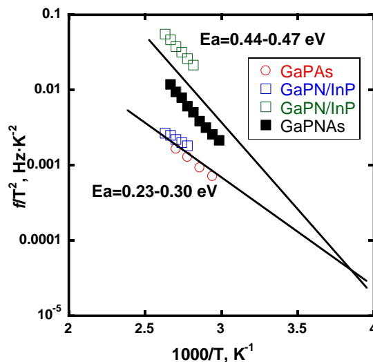
Figure 2. Arrhenius plot of f/T^2 for the defects identified by admittance spectroscopy for the GaPNAs, GaPN/InP and GaPNAs structures.
