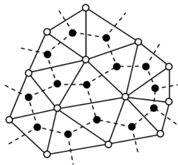
Figure 1: Simplex meshes and triangulations are topological but not geometrical duals. White dots: triangulation vertices ; Black dots: simplex mesh vertices.
