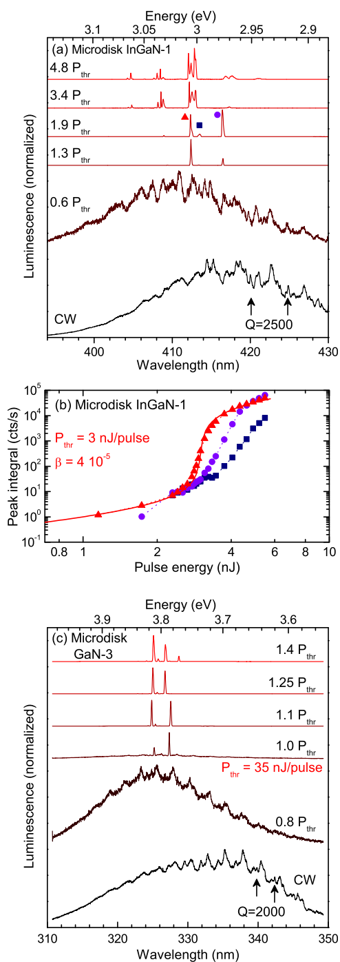
FIG. 2. (a) Photoluminescence spectra of a 4 \mu\text{m} microdisk in the sample InGaN-1, as a function of the pulsed laser excitation power; the CW spectrum of the same microdisk is presented for comparison. (b) Input-output characteristics of the 3 lasing modes marked on the panel (a); the symbols represent the peak integrals when the underlying 15 nm-broad background is subtracted; the plain red line shows the fit of the intensity of the first peak (triangles) by the microlaser rate equation model. (c) Photoluminescence spectra of a 6 \mu\text{m} microdisk in the sample GaN-3, as a function of the pulsed laser excitation power; the CW spectrum of the same microdisk is presented for comparison.
