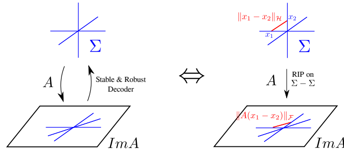
Fig. 1: A graphical representation of the equivalence between the existence of stable robust decoders and the RIP on the secant set. Operators satisfying the RIP approximately preserve distances between elements of \Sigma .
