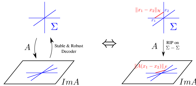
Fig. 1: A graphical representation of the equivalence between the existence of stable robust decoders and the RIP on the secant set. Operators satisfying the RIP approximately preserve distances between elements of \Sigma .
