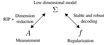
Fig. 2: Structure of the framework: the RIP framework allows to separate the study of dimension reduction and of decoding.
