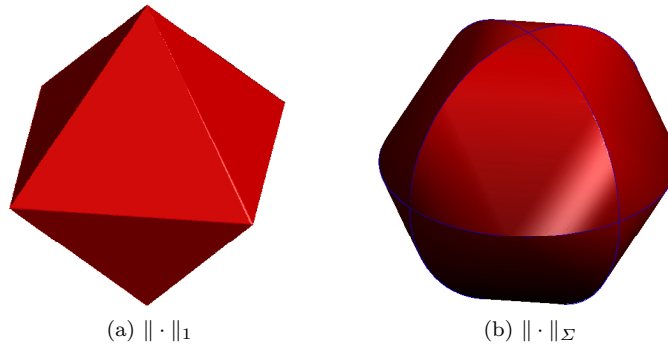
Fig. 7: The unit ball of \|\cdot\|_1 (left) and the unit ball of \|\cdot\|_{\Sigma} ( k -support norm) for \Sigma = \Sigma_2 the set of 2-sparse vectors in 3D (right).
