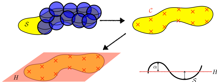
Fig. 6: Construction of H . Top left : cover of \mathcal{S} with N(\mathcal{S}, \alpha) balls of radius \alpha . Top right : the centers of the balls, indicated by the red crosses, form an \alpha -cover, denoted by \mathcal{C} , for \mathcal{S} . Bottom left : H is defined as the linear span of the vectors in \mathcal{C} . Bottom right : H approximates \mathcal{S} with precision \alpha .
