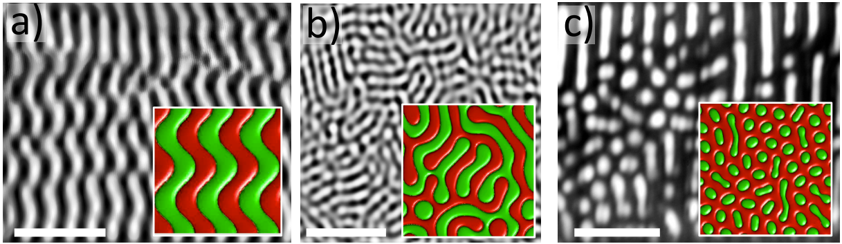
Figure 3. Eutectic growth patterns in bulk directional solidification. Real-time observations in transparent alloys with the DIRSOL setup: a) Zigzag pattern ( \text{CBr}_4\text{-C}_2\text{Cl}_6 ; V = 0.39\mu\text{ms}^{-1} ); note the presence of defects reminiscent of the fault lines commonly observed in bulk metallic eutectics [26]. b) Labyrinth pattern ( \text{CBr}_4\text{-C}_2\text{Cl}_6 ; V = 1.0\mu\text{ms}^{-1} ) [41]. c) Coexistence between rods, elongated rods and broken lamellae ( \text{SCN-DC} ; V = 0.01\mu\text{ms}^{-1} ) [42]. Bars: 100\mu\text{m} . Insets: 3D phase-field calculations (eutectic alloy with symmetric phase diagram) [39,43].
