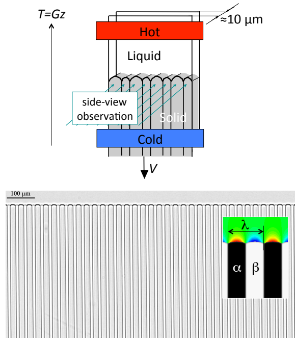
Figure 1. Top: Principle of thin-sample directional solidification. V : pulling velocity. G : temperature gradient (vertical axis z ). Side-view observation: optical microscope. Bottom: Steady periodic (lamellar) eutectic growth pattern in thin-sample directional solidification (slightly hypereutectic \text{CBr}_4\text{-C}_2\text{Cl}_6 transparent alloy; V = 1 \mu\text{m.s}^{-1} ; \lambda \approx 1.2\lambda_{JH} ). Liquid and solid-solid interfaces are seen as dark lines. Inset: Two-dimensional phase-field numerical simulation of a periodic lamellar pattern (model symmetric eutectic alloy). \alpha and \beta : solid phases. Colors in the liquid: solute diffusion field. \lambda : lamellar spacing.
