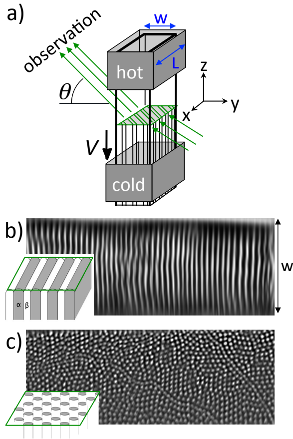
Figure 2. a) Principle of the DIRSOL apparatus for real-time, oblique-view observation (viewing angle \theta ) of the solid-liquid interface with a long-distance optical microscope during directional solidification of transparent eutectic alloys. y : normal to the glass walls. w and L : thickness and lateral width of the sample ( L \gg w ). b) Lamellar pattern; near-eutectic \text{CBr}_4\text{-C}_2\text{Cl}_6 alloy ( V = 0.37 \mu\text{m s}^{-1} ; w = 350 \mu\text{m} ). Bright (dark) lamellae: \alpha ( \beta ) phase. c) Rod-like pattern in a 350\text{-}\mu\text{m} sample of a near-eutectic succinonitrile-d,camphor alloy ( V = 0.035 \mu\text{m s}^{-1} ). Bright spots: DC fibers in the (dark) SCN matrix. The images have been rescaled numerically to 1:1 aspect ratio. Insets: schematic perspective of the two kinds of growth patterns.
