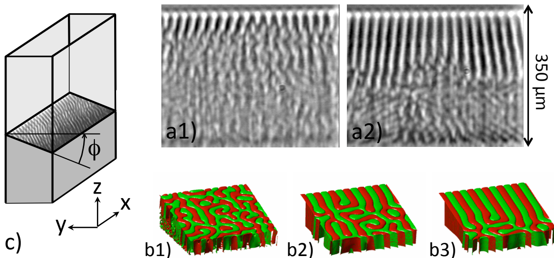
Figure 4. Real-time observations: a1) and a2) Global drift of a labyrinth pattern and formation of regular lamellae by an invasion process due to a thermal-bias effect. b1) to b3): Phase field simulations of this morphological transition at three successive instants (thermal-bias angle \phi = 12^\circ ). c) Schematic representation of the thermal bias.
