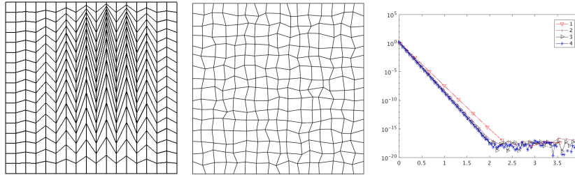
Fig. 2 Left: First Kershaw mesh. Middle: Third quadrangle mesh. Right: Discrete relative energy \mathbb{E}_{\mathcal{T}}^n - \mathbb{E}_{\mathcal{T}}^{\infty} as a function of n\Delta t computed on the first four Kershaw meshes.
