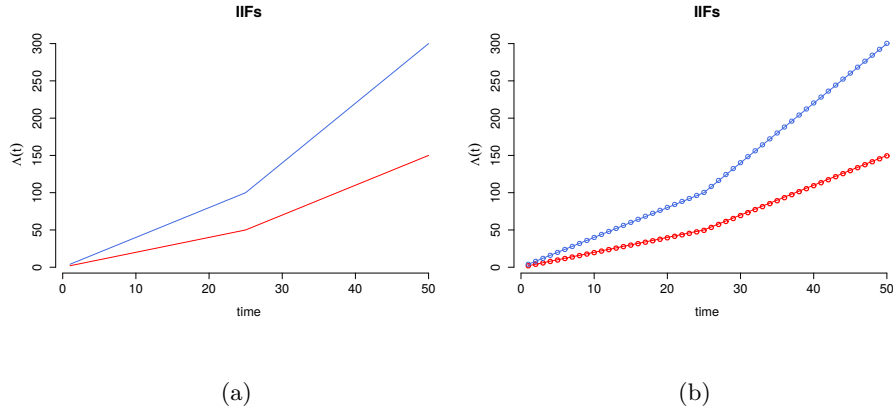
Figure 3: Real 3a and estimated 3b integrated intensity functions (IIFs) according to the considered generative model. In blue we have \Lambda_1(t) , for \psi = 4 , in red \Lambda_2(t) .
