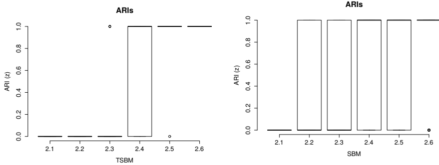
(b) ARIs obtained with the Gibbs sampling procedure for SBM.
