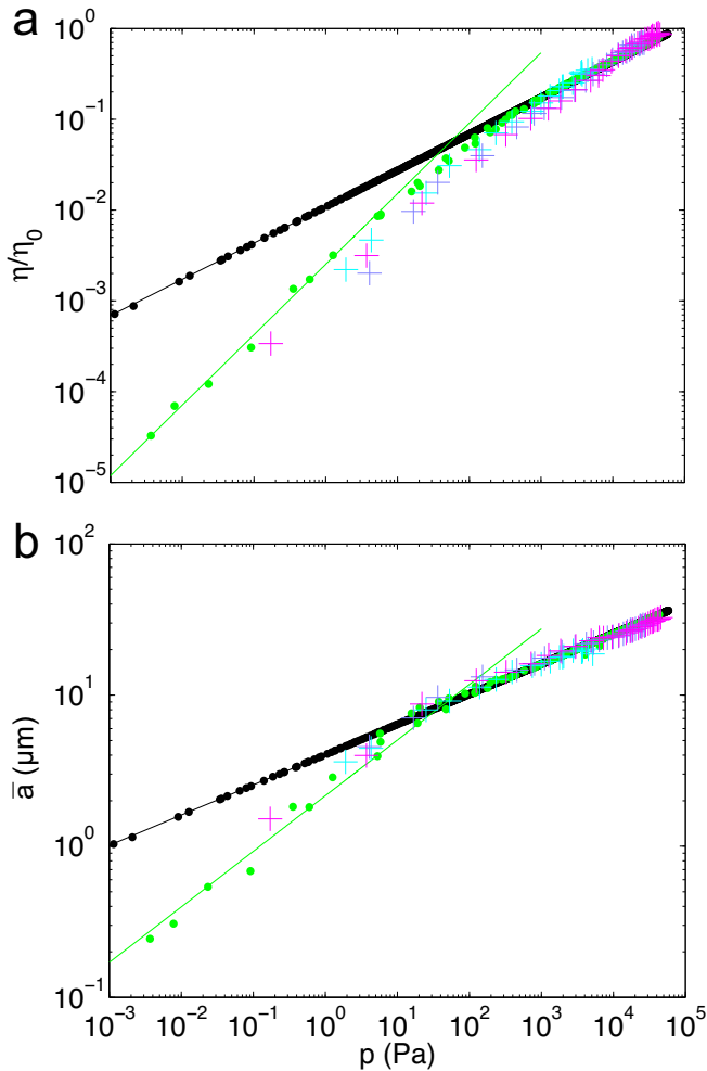
FIG. 7: (Color online) (a) Microcontacts density \eta , normalized by the mean number of micro-asperities per unit area \eta_0 , versus local pressure p for the SA sample with \phi = 0.4 . (b) Mean microcontacts area \bar{a} versus local pressure p for the same sample. On both graphs, black disks are the results of GT's model predictions, the green disks are predictions of Ciaravella et al. 's model with \alpha_{ij} \neq 0 and crosses correspond to the experimental data at three different loads P = 0.02, 0.2, 0.5 N. Thick black lines are power law fits of GT's model predicted data, while green solid lines are power law fits of Ciaravella et al. 's model predicted data for p < p^* , with p^* \approx 50 Pa.
