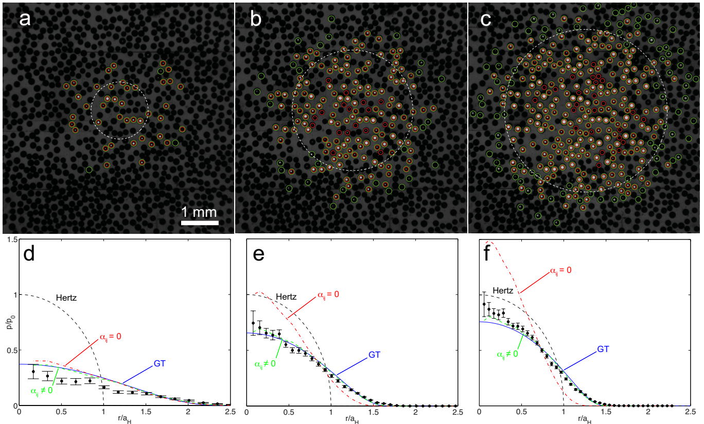
FIG. 6: (Color online) (a), (b), (c) Images of the interface at P = 0.02, 0.2, 0.5 N with the \phi = 0.4 SA sample. microcontacts appear as the white disks. Green ( resp. red) circles indicate Ciaravella et al. 's model predicted microcontacts with \alpha_{ij} \neq 0 ( resp. \alpha_{ij} = 0 ). On all images, the white dashed line circles delimit Hertz contacts for the corresponding P . (d),(e),(f) Angularly averaged pressure p distribution as a function of the distance to the center r on a SA sample with \phi = 0.4 at increasing normal loads P . Both p and r are normalized by respectively, Hertz' maximum pressure p_0 and Hertz contact radius a_H . The black dashed line corresponds to Hertz prediction. Blue solid lines are fits using Greenwood-Tripp model (GT) with a uniform asperity height density and same surface density \phi . The red dot-dashed lines are predictions of Ciaravella et al. 's model [14, 15] setting the interaction term \alpha_{ij} = 0 , while the green dashed lines correspond to the full model with \alpha_{ij} \neq 0 . Both latter predictions are statistical averages over 1000 independent pattern realizations with \phi = 0.4 and a uniform height distribution.
