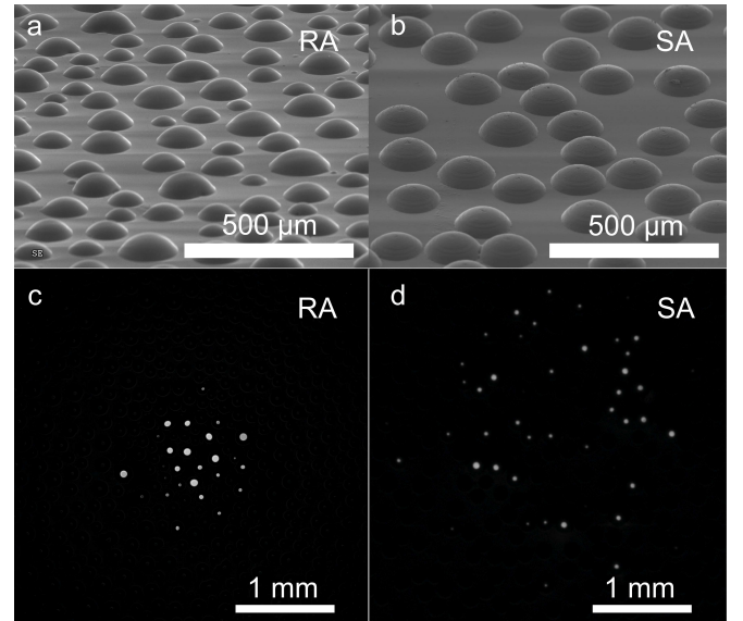
FIG. 1: (a) SEM image topography of a \text{RA}^+ sol-gel replica ( \phi = 0.41 ). (b) Same with an SA PDMS replica of a micro-milled mold ( \phi = 0.4 ). (c) microcontacts spatial distribution with \text{RA}^+ ( P = 22 \text{ mN} ). (d) Same with the SA of (b) and a lens of radius of curvature 128.8 mm ( P = 20 \text{ mN} ). (c-d) are image differences with a reference non-contact image. Note the size difference in the apparent contact related to the difference in curvature of both indenters.
