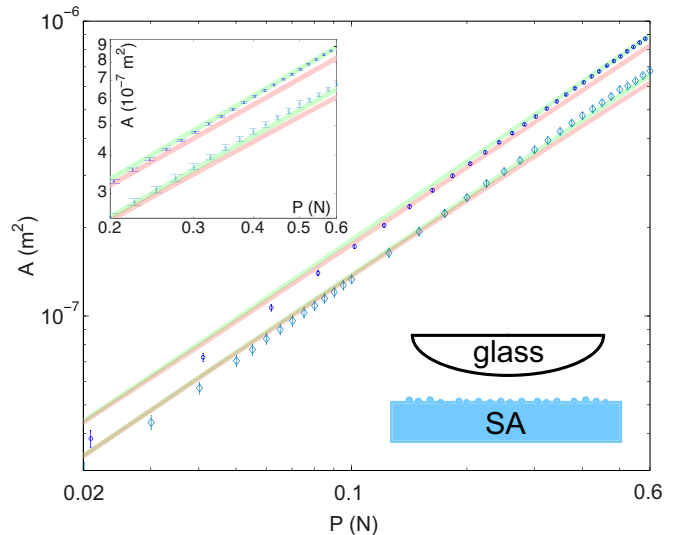
FIG. 5: Log-log plot of the real area of contact A versus P for both SA^- ( \phi = 0.1 , blue diamonds) and SA^+ ( \phi = 0.4 , blue circles) samples. The inset is a close up for 0.2 \leq P \leq 0.6 N. Error bars are given by the standard deviation of A on 24 different contact configurations. Red shaded areas correspond to the predictions of Ciaravella et al. 's model [14, 15] by setting \alpha_{ij} to 0 in eqn (2). Green areas correspond to \alpha_{ij} \neq 0 . Areas extent characterizes the scatter in the simulations, arising from uncertainties in the experimental determination of E .
