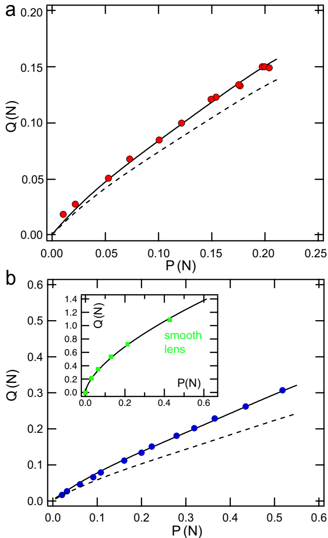
FIG. 8: Q versus P in steady sliding ( v = 0.5 \text{ mm s}^{-1} ) for contacts between a smooth PDMS substrate and \text{RA}^- (a) and \text{RA}^+ (b) lenses. On both graphs, dashed lines are the theoretical Q given by eqn (4), taking for A its measured values and for \tau_0 = 0.34 \text{ MPa} the average shear stress obtained with the smooth lens. Solid lines are fits of the experimental data with eqn (4), yielding \tau_0 = 0.40 \text{ MPa} for \text{RA}^- and 0.49 \text{ MPa} for \text{RA}^+ . Inset: Q versus P for the smooth lens, in steady sliding. The solid line is a fit of the data using eqn (4), taking for A its measured value in steady sliding.
