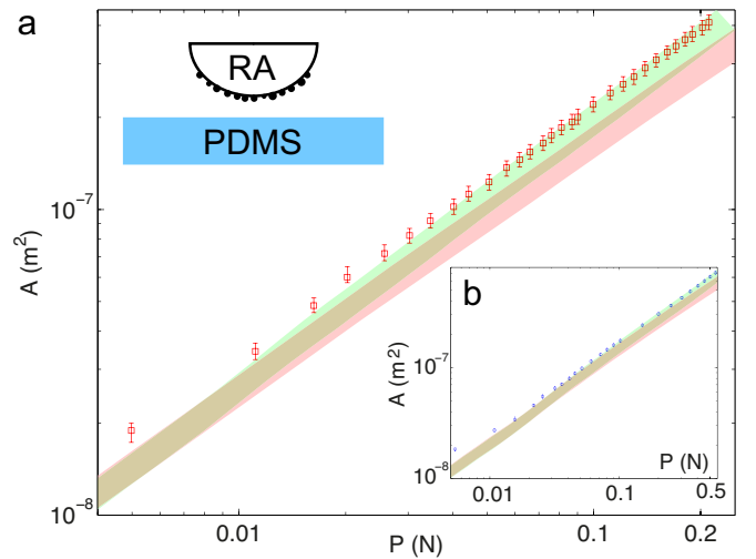
FIG. 4: Log-log plot of the real area of contact A versus P for both RA^- (a) and RA^+ (b) lenses. The upper and lower limits of the error bars correspond to the total areas measured with the arbitrarily chosen extremal values of the optical threshold (see text). Red shaded areas correspond to the predictions of Ciavarella et al. 's model [14, 15] by setting \alpha_{ij} to 0 in eqn (2). Green areas correspond to \alpha_{ij} \neq 0 . Areas extent characterizes the scatter in the simulations, arising from uncertainties in the experimental determination of the topography parameters.
