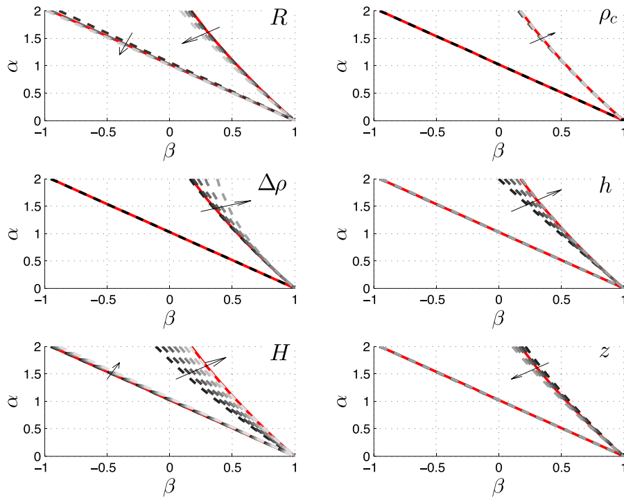
Figure 4. Sensitivity of the compensation degree ( \alpha_{\max} and \alpha_{\min} ) to model parameters. Parameters set: cylinder radius R , crustal density \rho_c , crust–mantle density contrast \Delta\rho , elevation h , reference crustal thickness H and satellite elevation z . Parameter ranges: R_{\min} \in [25; 100 \text{ km}] , R_{\max} \in [250; 1000 \text{ km}] , \rho_c \in [2600; 2900 \text{ kg m}^{-3}] , \Delta\rho \in [-700; -300 \text{ kg m}^{-3}] , h_{\min} \in [0; 1 \text{ km}] , h_{\max} \in [1; 5 \text{ km}] , H_{\min} \in [10; 25 \text{ km}] , H_{\max} \in [30; 60 \text{ km}] and z \in [230; 270 \text{ km}] . The grey colour scale (dashed lines) and associated black arrows indicate an increase in the parameter value. The red lines are associated with the data collection presented in Fig. 3.
