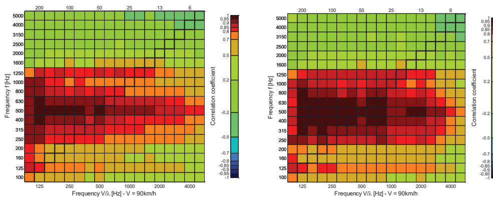
Figure 16 - Maps of correlation coefficients evaluated between third-octave enveloped texture levels and CB noise levels – Left : 2D enveloped road texture – Right : 3D enveloped combined tyre/road roughness
