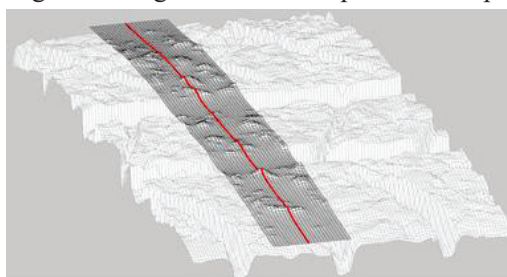
Figure 11 – Loaded sliding rubber block (in black) moving over the combined tyre/road roughness (in white) and selected transverse profile (in red)
