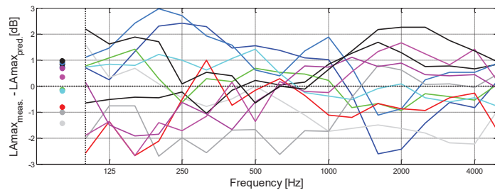
Figure 18 – Prediction errors on third-octave CB levels at 90 km/h
