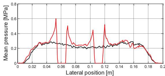
Figure 13 – Contact pressure averaged over the rolling direction - Red curve: patterned E3A tyre – Black curve: slick tyre
