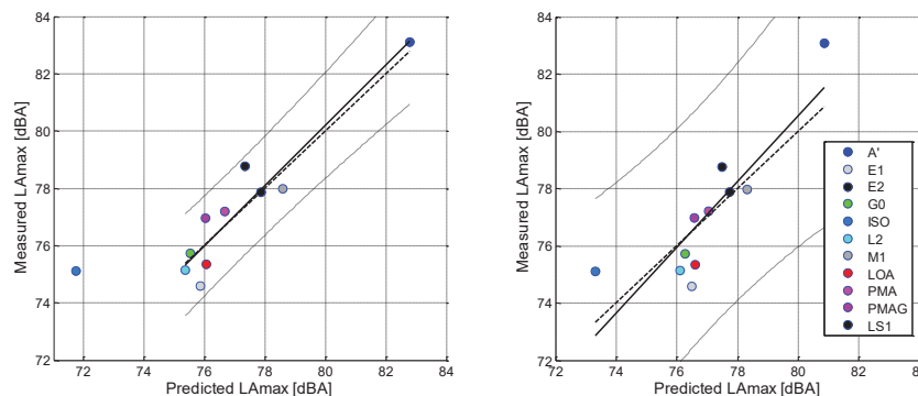
Figure 4 – Relationship between predicted and measured LAmax at 90 km/h reconstructed from third-octave
