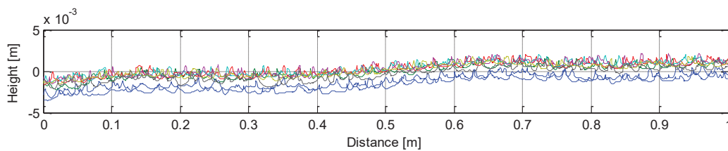
Figure 14 – Examples of longitudinal profiles extracted from the enveloped surface
