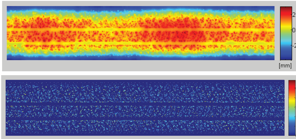
Figure 12 – Top: enveloped tyre/road combined roughness –Bottom: pressure map
