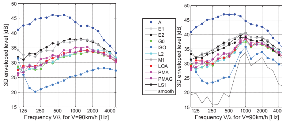
Figure 15 – 3D combined enveloped roughness levels as a function of time frequency for V=90 km/h – Left: slick tyre – Right: patterned tyre
