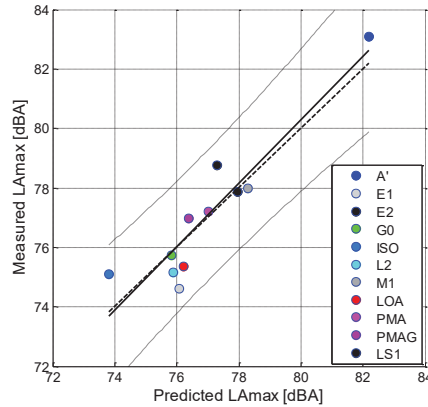
Figure 17 – Relationship between predicted and measured LAmax at 90 km/h reconstructed from third-octave CB levels
