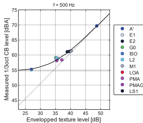
Figure 5 – Relationship between third-octave levels at 500 Hz and 90 km/h and enveloped texture levels
