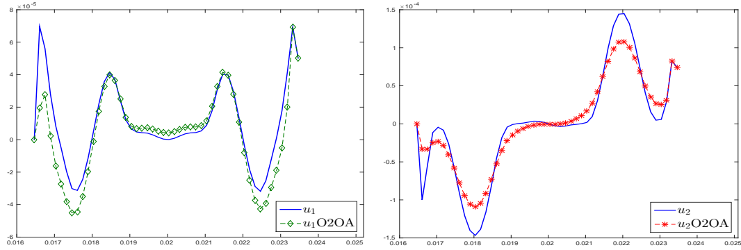
Figure A.15: Application: The reconstructed velocity on \Gamma_1 (With stent).
