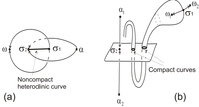
Figure 1: Heteroclinic curves
