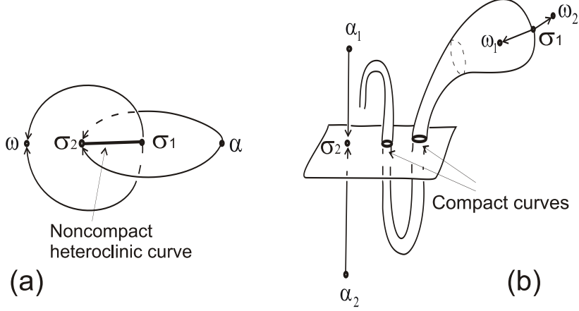
Figure 1: Heteroclinic curves
