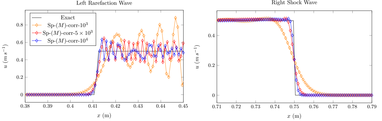
Figure 13: Velocity profile at M = 4.2 \times 10^{-3} , Sp-(M)-corr
