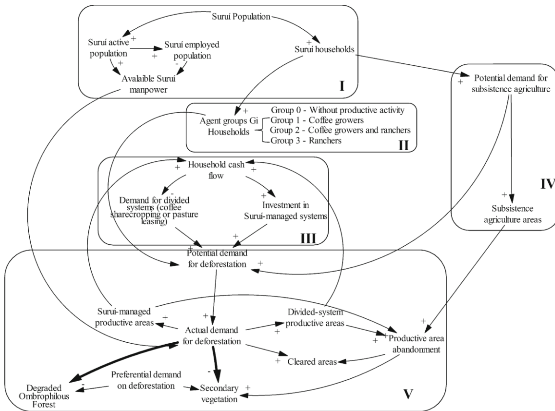
SUB-MODEL I : DEMOGRAPHICS SUB-MODEL II : PRODUCTIVE AGENTS SUB-MODEL III : ECONOMIC DYNAMICS OF PRODUCTIVE -AGENT GROUPS SUB-MODEL IV : SUBSISTENCE AGRICULTURE SUB-MODEL V : LANDSCAPE DYNAMICS
