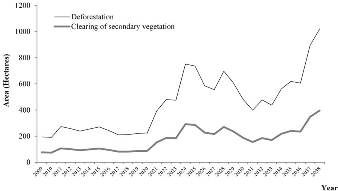
Fig. 6 Landscape dynamics through SIMSURUI simulations between 2009 and 2038
