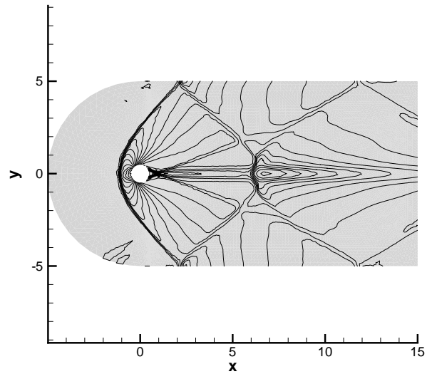
Figure 19: Mach number isolines for test case 4.3.
