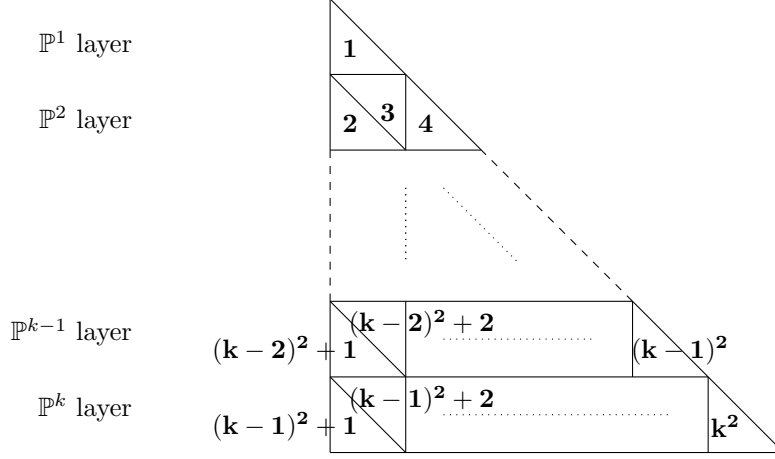
Figure 7: Numbering of \mathbb{P}^1 sub-triangles constituting the bottom face of the \mathbb{P}^k layer of tetrahedron K .
