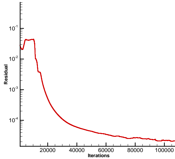
Figure 23: Convergence of residual for test case 4.4
