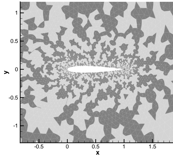
Figure 10: Mesh for test case 4.1 with elements randomly subdivided: elements in dark zones are subdivided, the others are not subdivided.
