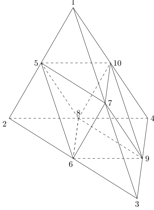
Figure 2: Subdivided tetrahedron K .
