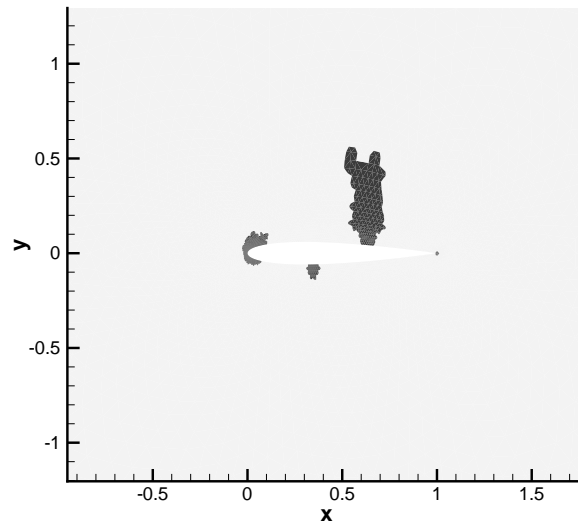
Figure 12: Shock zone for test case 4.2: subdivided elements are dark-colored.
