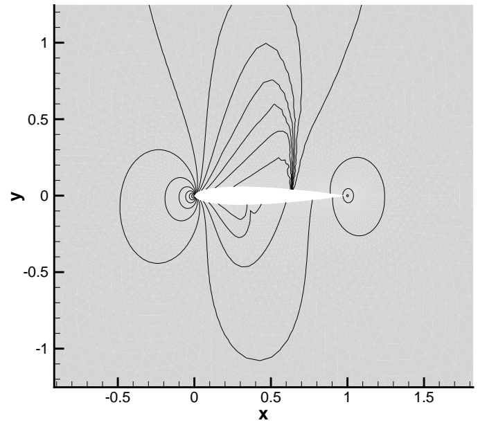
(b) Pressure ( \mathbb{P}^2 elements)
