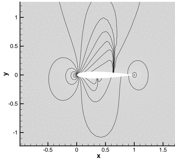
(c) Pressure (mixed elements)
