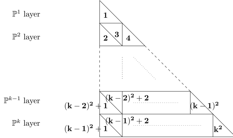
Figure 4: Ordering of vertices for relation (47).
