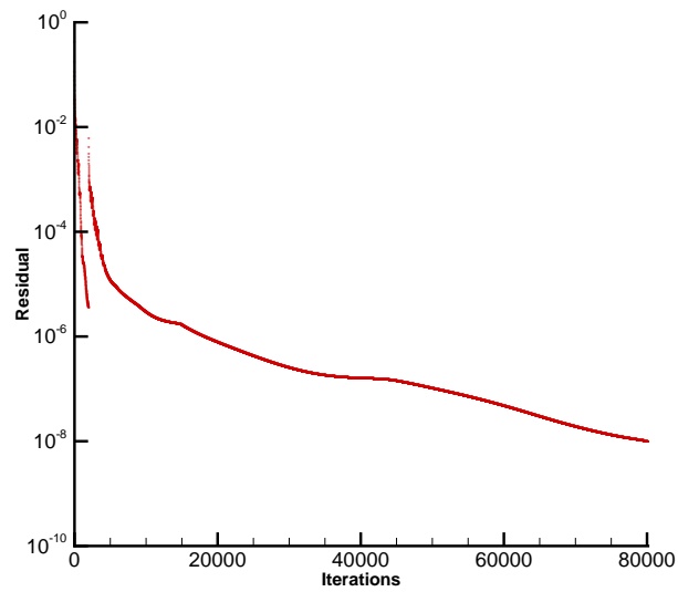
Figure 13: Convergence of residual for test case 4.2 with mixed elements.
