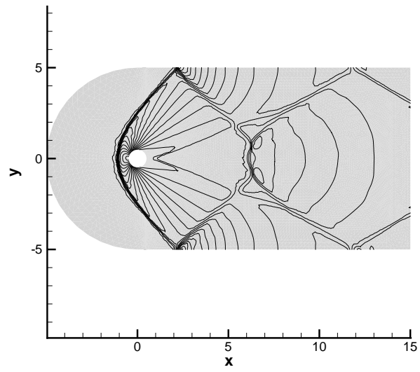
Figure 20: Pressure isolines for test case 4.3.
