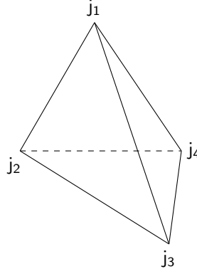
Figure 8: Ordering of vertices
