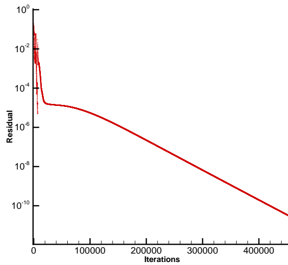
Figure 18: Convergence of residual in test case 4.3.
