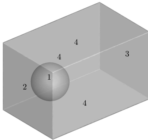
Figure 22: Boundaries for test case 4.4.
