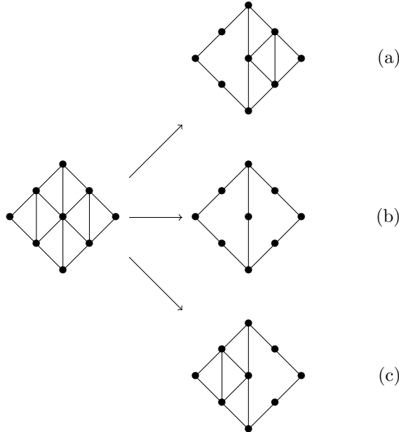
Figure 9: Possible transformations of two adjacent (initially subdivided) triangles. Notice that no hanging node is generated.
