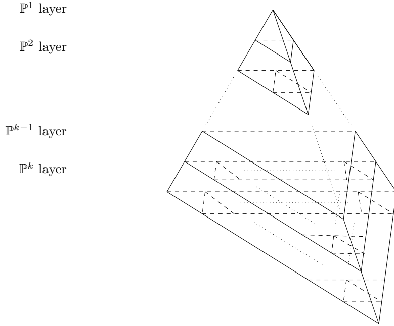
Figure 6: Subdivided \mathbb{P}^k tetrahedron K : layers and their bottom faces.
