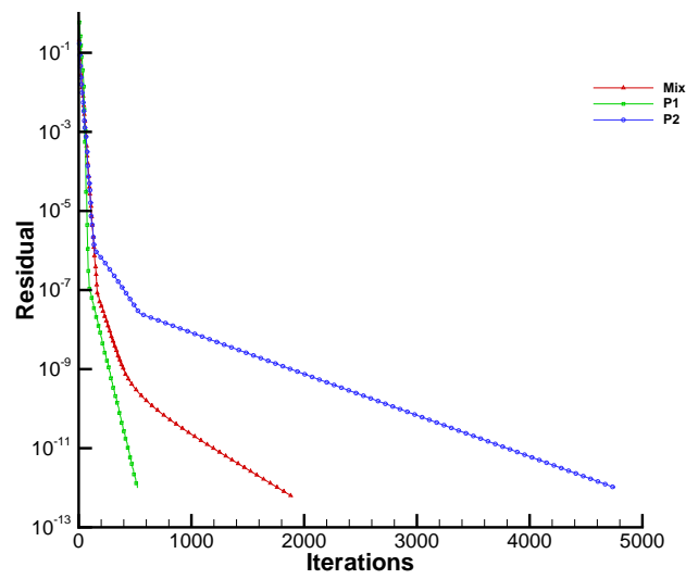
Figure 11: Convergence of residuals for test case 4.1.
