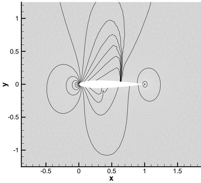
(a) Pressure ( \mathbb{P}^1 elements)
