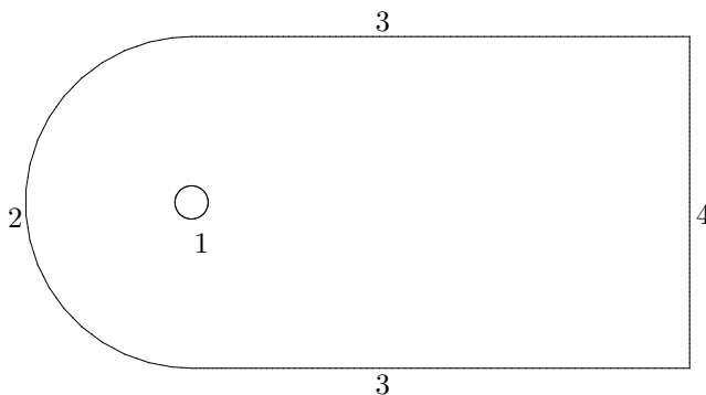
Figure 16: Boundaries for test case 4.3.
