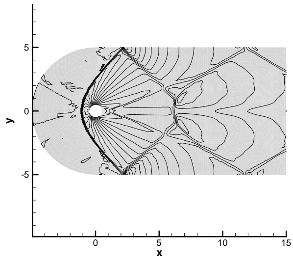
Figure 21: Density isolines for test case 4.3.
