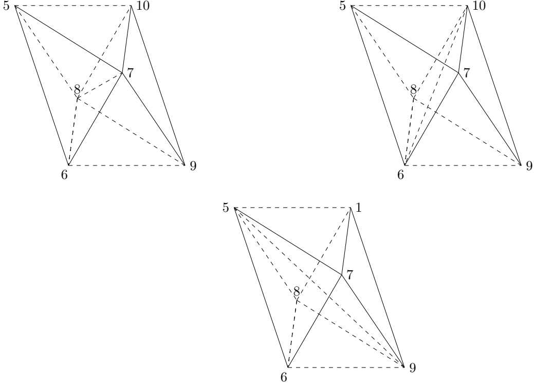
Figure 3: Subdivided octahedron with resp. diagonal (8,7),(10,6) and (5,9).
