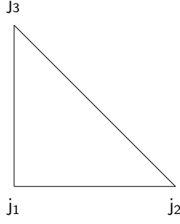
Figure 4: Ordering of vertices for relation (47).
