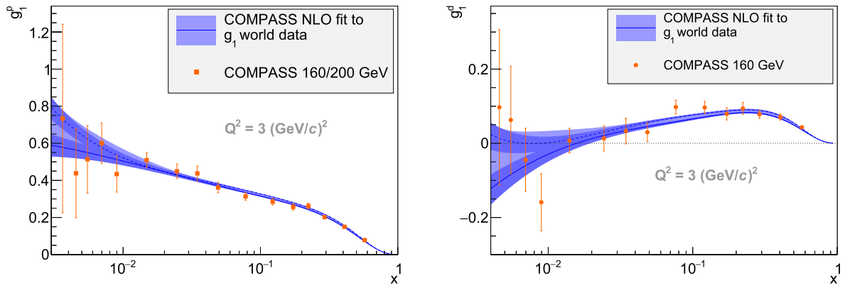
Fig. 6. Results of the QCD fits to g_1^p (left) and g_1^d (right) world data at Q^2 = 3 \text{ (GeV/c)}^2 as functions of x . The curves correspond to the two sets of functional shapes as discussed in the text. The dark bands represent the statistical uncertainties associated with each curve and the light bands, which overlay the dark ones, represent the total systematic and statistical uncertainties added in quadrature. (Coloured version online.)
