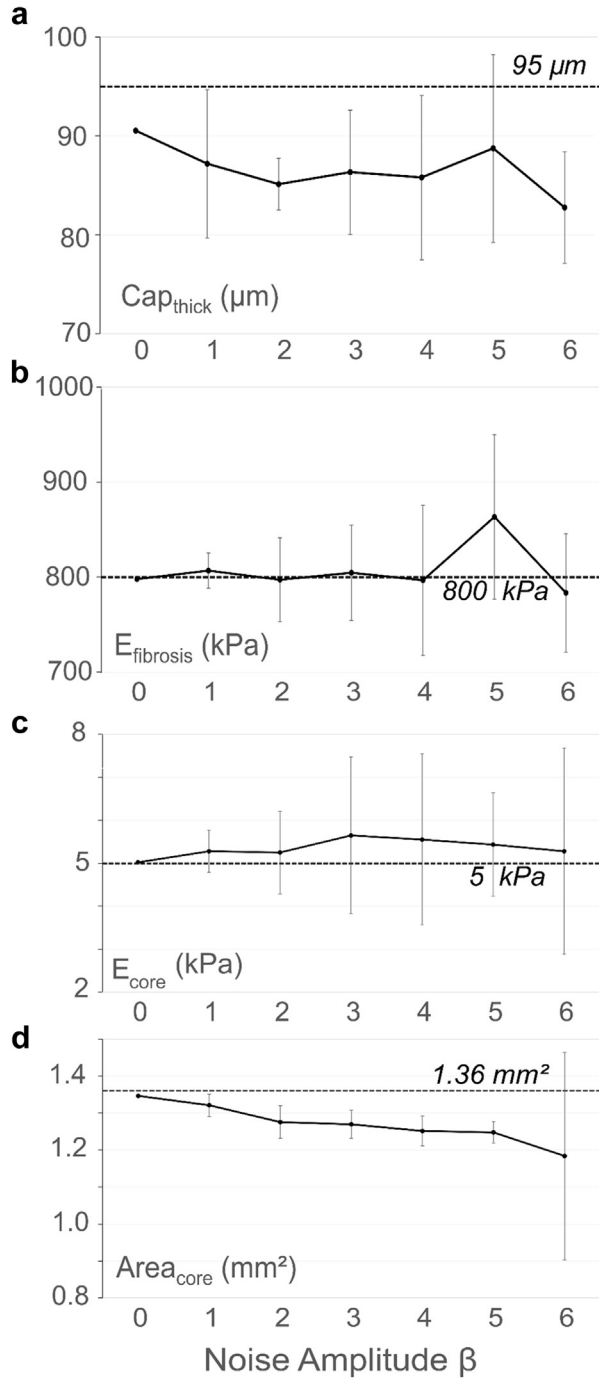
Fig. 8. Influence of white noise amplitude on estimations of cap thickness ( \text{Cap}_{\text{thick}} ), Young's moduli of the necrotic core ( E_{\text{core}} ) and fibrosis ( E_{\text{fibrosis}} ) and necrotic core area ( \text{Area}_{\text{core}} ). Plaque #2 was used for this investigation. Knowing that the noise was spatially randomly distributed, we performed 20 computations for each amplitude of noise \beta and present the mean values \pm the standard deviations. The dashed lines indicate the values used for the forward problem. (a) Influence of noise on \text{Cap}_{\text{thick}} estimation. (b) Influence of noise on E_{\text{fibrosis}} estimation. (c) Influence of noise on E_{\text{core}} estimation. (d) Influence of noise on \text{Area}_{\text{core}} estimation.
