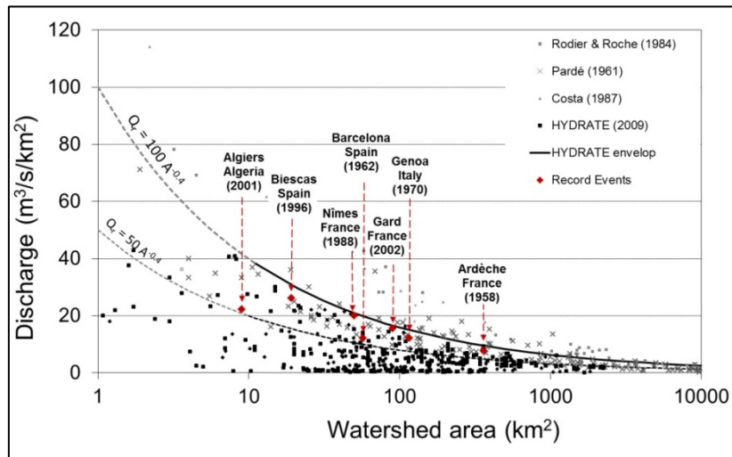
Figure 2. Reported estimated world records from different sources, proposed European envelope curve and some selected European record events since 1940
