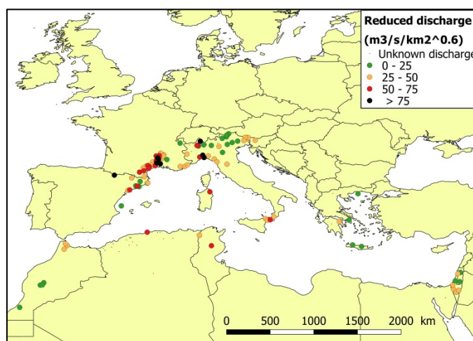
Figure 4. Estimated reduced peak discharge of the documented flood events over the period 1940-2015. The reduced discharge Q_r is Q/A^{0.6} , Q is the peak discharge ( m^3/s ) and A is the watershed area ( km^2 ).
