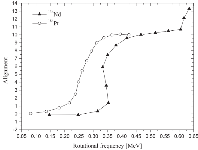
FIG. 10. Experimental alignments for ^{134}\text{Nd} and ^{184}\text{Pt} . Harris reference parameters of \mathcal{I}_0 = 17.0\hbar^2 \text{ MeV}^{-1} and \mathcal{I}_1 = 25.0\hbar^2 \text{ MeV}^{-1} (the same as in Ref. [3]) were used for both nuclei.
