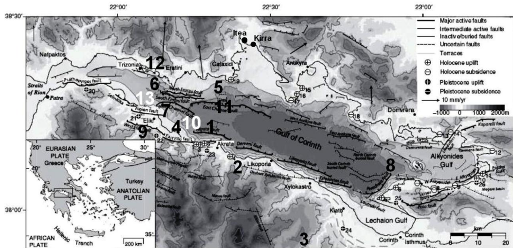
Fig. 1. Map of the Corinth Rift showing topography, bathymetry and faults (after Bell et al., 2009 and references therein). Inset box shows the location of the rift inside the Aegean region. The large figures from 1 to 13 indicate the locations of the tsunami sources discussed in the text and arranged according to their year of occurrence of the tsunamis as: 373 BC (1), AD 1402 (2), 1742 (3), 1748 (4), 1794 (5), 1817 (6), 1861 (7), 1887 (8), 1888 (9), 1963 (10), 1965 (11), 1995 (12), 1996 (13). Detailed references for each one of the 13 tsunami sources can be found in Papadopoulos (2003). Black figures show seismic sources, white show aseismic earth slump sources. The test-site of Kirra is shown at the north coast. The test-site of Aliki is situated very close to source n. 7. Figures attached to uplift and subsidence are in cm.
