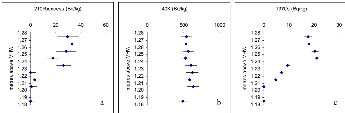
Fig. 8. Results of radiometric dating in trench 1, Kirra: variation in ^{210}\text{Pb} (a), ^{40}\text{K} (b) and ^{137}\text{Cs} (c) with depth.
