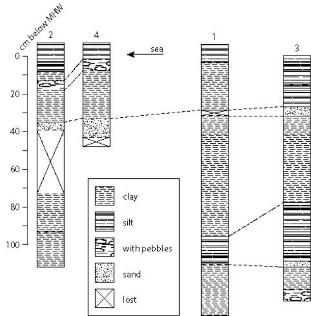
Fig. 7. Lithostratigraphy of Aliki. Cores 2 and 4 are located at the seaward side of the lagoon just behind the barrier and cores 1 and 3 at the landward side.
