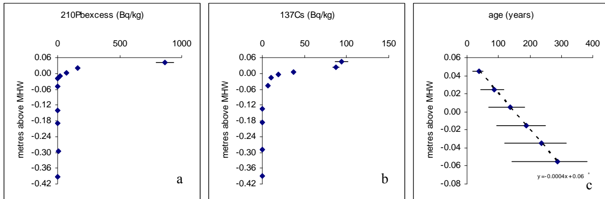
Fig. 9. Results of radiometric dating in core 4, Aliko: variation of ^{210}\text{Pb} (a) and ^{137}\text{Cs} (b) with depth and the sediment accumulation rate (age-depth curve) based on the simple model of ^{210}\text{Pb} dating (c).
