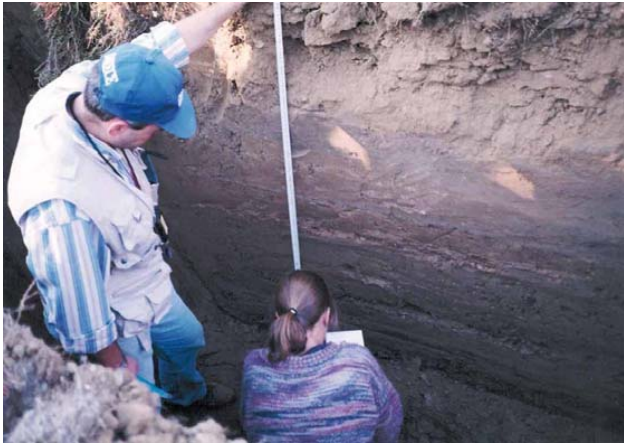
Fig. 4. One of trenches opened in Kirra.
