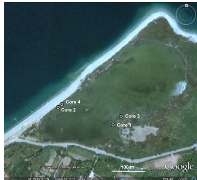
Fig. 3. The field site of Aliko lagoon from a Google image.
