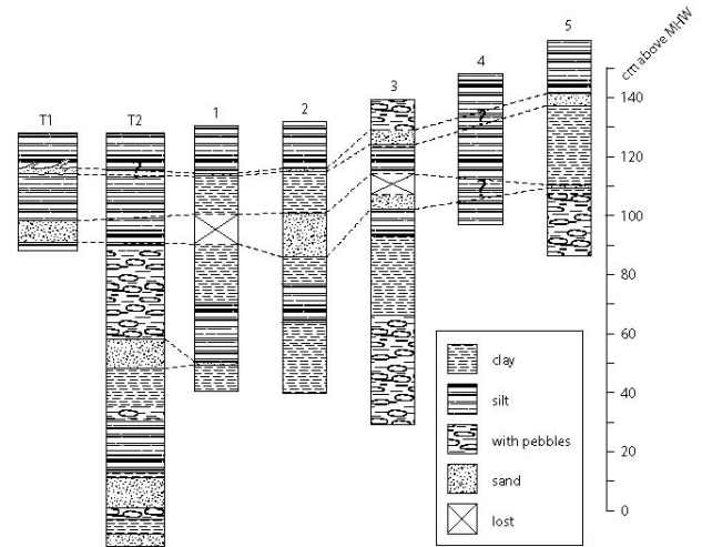
Fig. 6. Lithostratigraphy of Kirra in two trenches (T1 and T2) and five cores.
