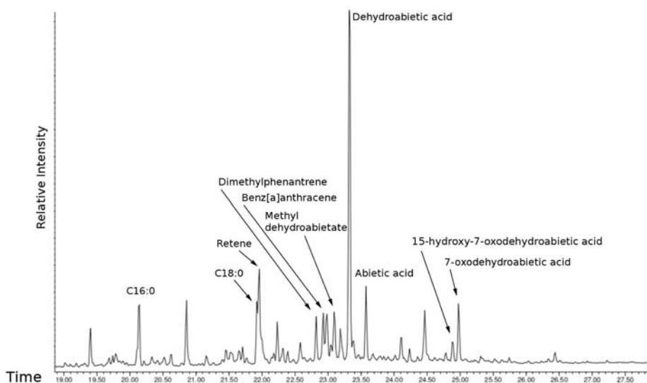
Figure 5 - Partial total ion chromatogram of the lipid extraction of Keay 25.1 sample AIX/64 (I84LIP).
