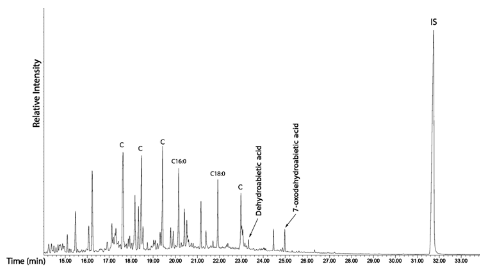
Figure 6 - Partial total ion chromatogram of the lipid extraction of Keay 25.1 sample AIX/66 (I93LIP), 'C' represents contaminants.
