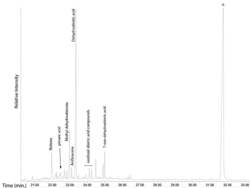
Figure 4 - Partial total ion chromatogram of a sample of visible pitch from Keay 25.1 sample AIX/51 (I72LIP).
