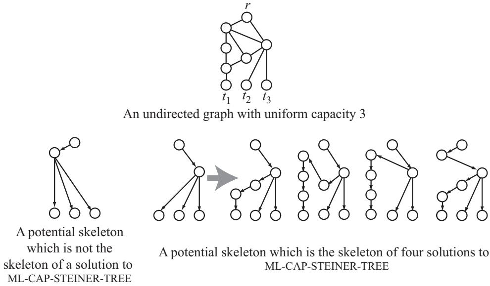
Figure 2: Potential skeletons in a graph G .
