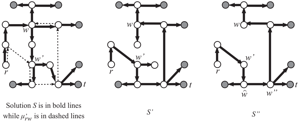
Figure 8: Illustration of the proof of Claim 7.7.
