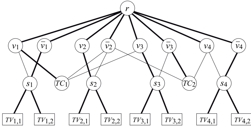
Figure 7: From 3\text{-SAT}_3 to \text{CAP-STEINER-TREE} .
